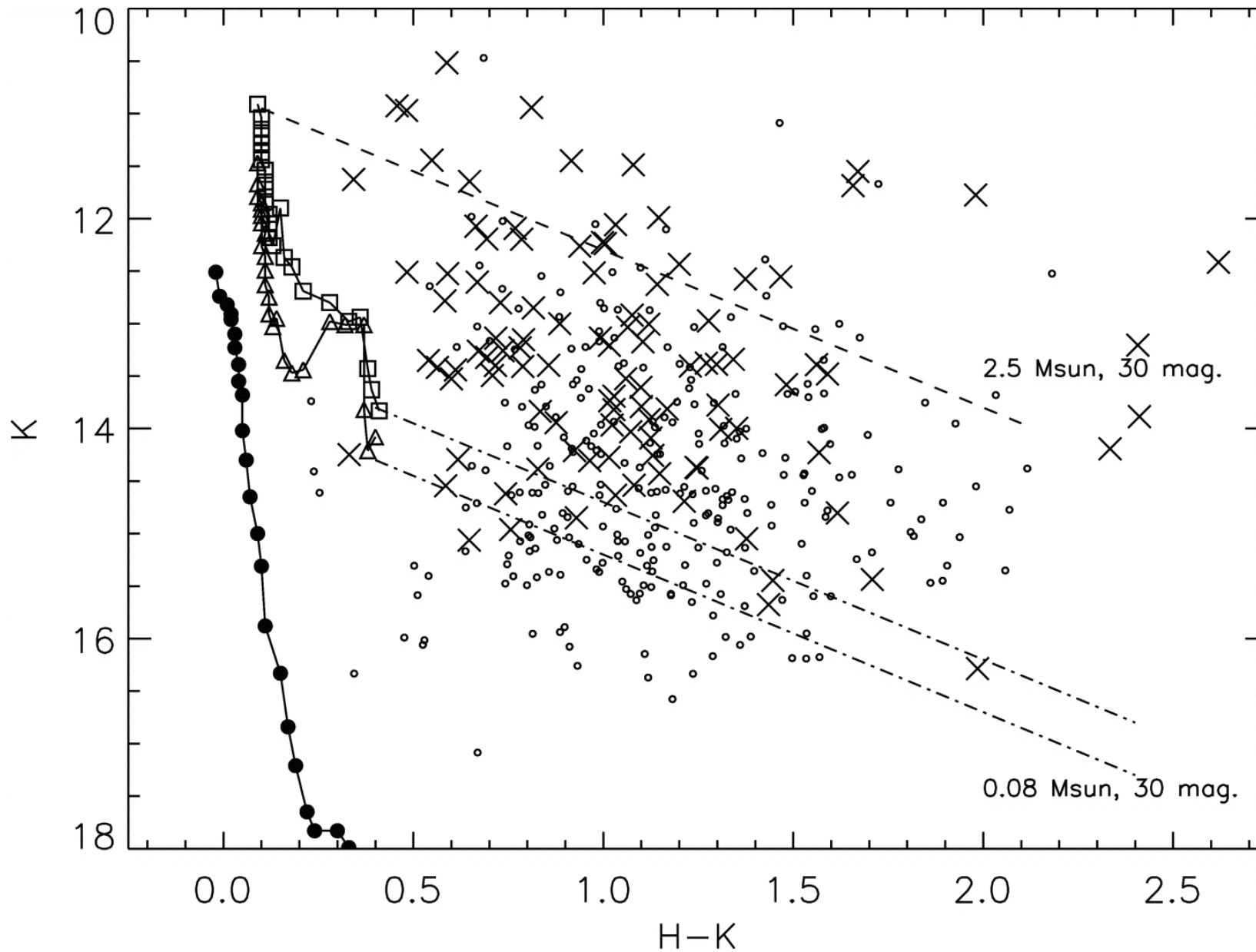
Fig. 16. from XRay and Infrared Point Source Identification and Characteristics in the Embedded, Massive StarForming Region RCW 38 Wolk et al. 2006 AJ 132 1100 doi:10.1086/505704 https://dx.doi.org/10.1086/505704
