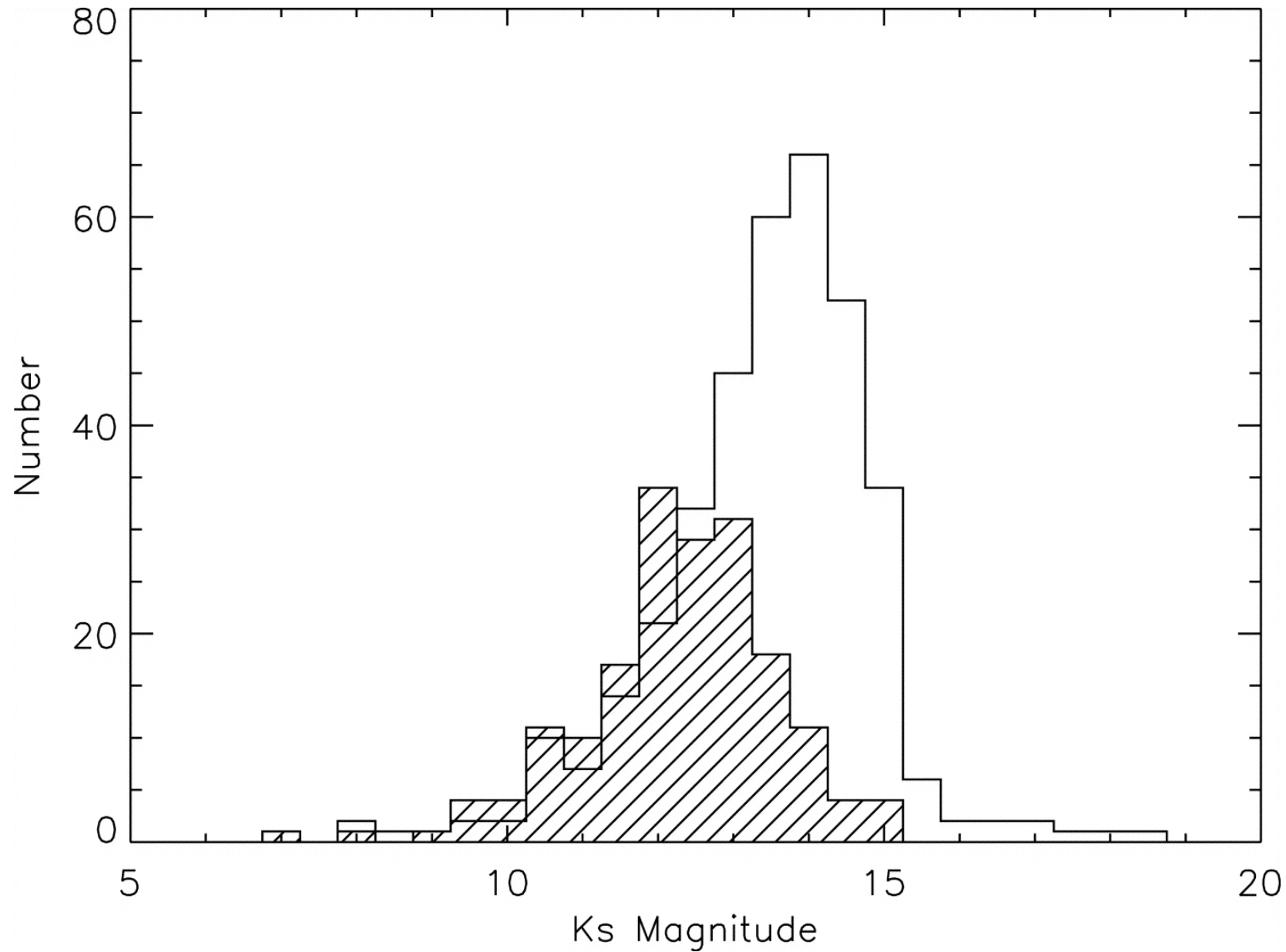
Fig. 15. from XRay and Infrared Point Source Identification and Characteristics in the Embedded, Massive StarForming Region RCW 38 Wolk et al. 2006 AJ 132 1100 doi:10.1086/505704 https://dx.doi.org/10.1086/505704 © 2006. The American Astronomical Society. All rights reserved. Printed in U.S.A.
