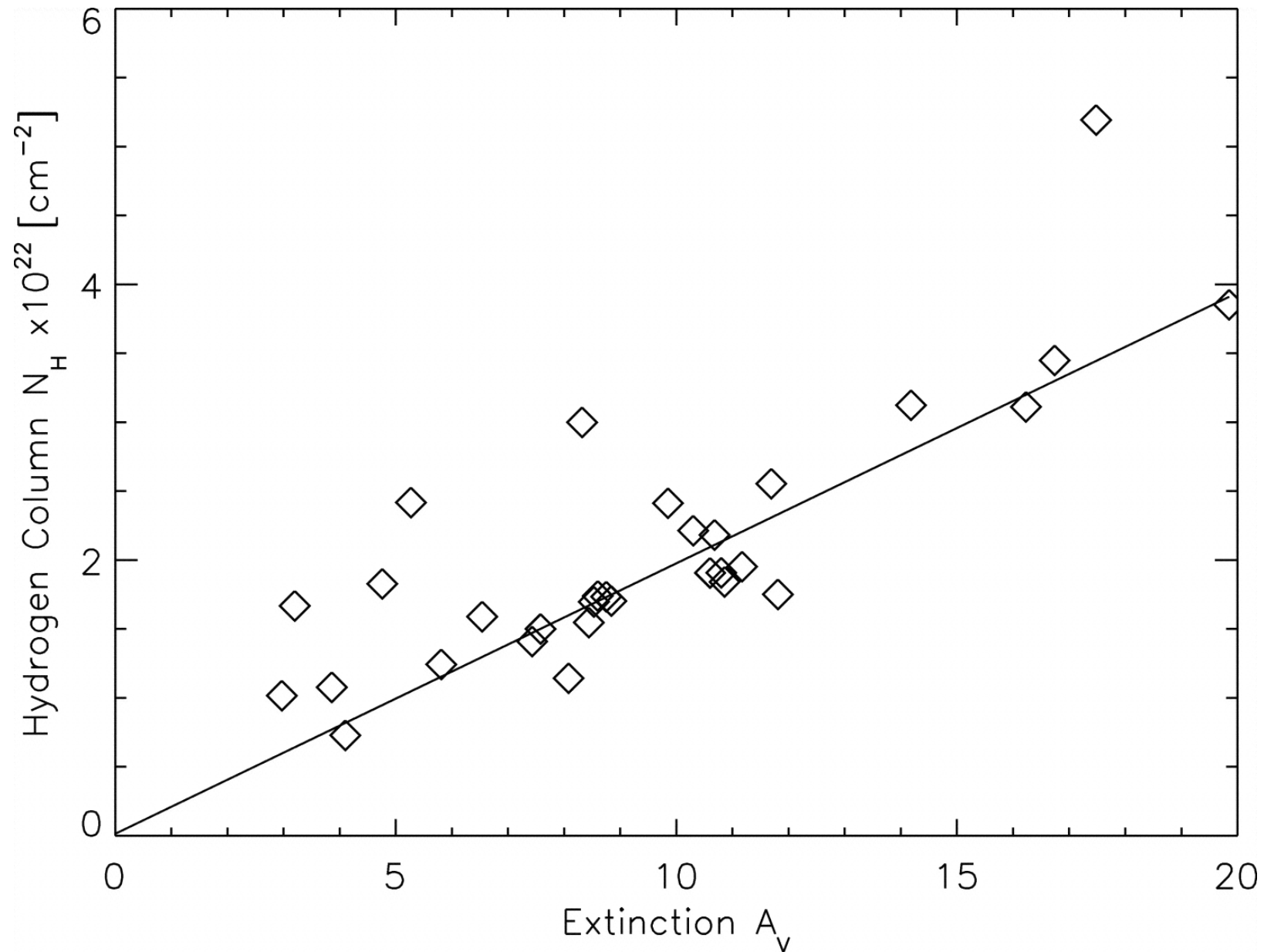
Fig. 14. from XRay and Infrared Point Source Identification and Characteristics in the Embedded, Massive StarForming Region RCW 38 Wolk et al. 2006 AJ 132 1100 doi:10.1086/505704 https://dx.doi.org/10.1086/505704
