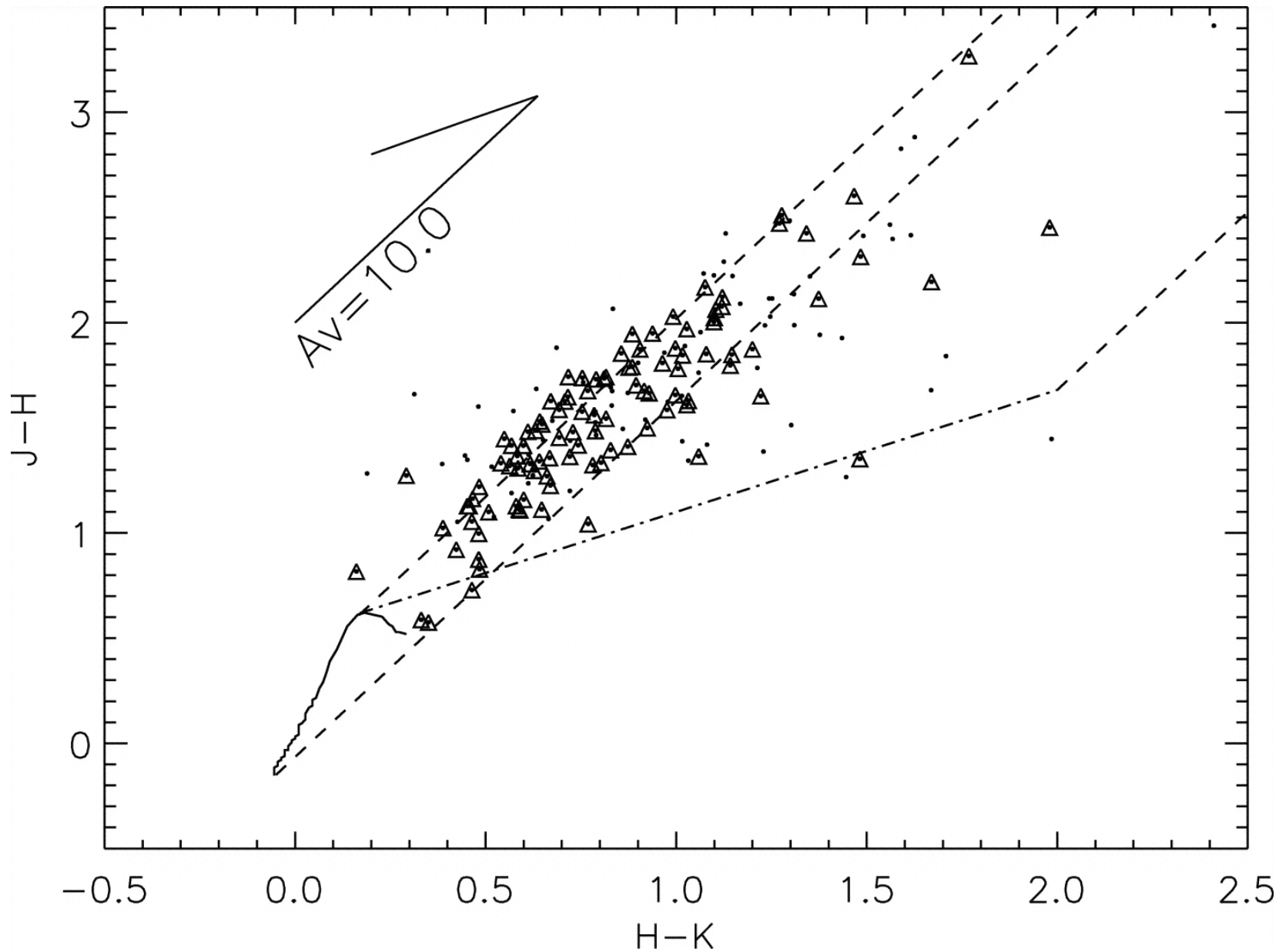
Fig. 13. from XRay and Infrared Point Source Identification and Characteristics in the Embedded, Massive StarForming Region RCW 38 Wolk et al. 2006 AJ 132 1100 doi:10.1086/505704 https://dx.doi.org/10.1086/505704 © 2006. The American Astronomical Society. All rights reserved. Printed in U.S.A.
