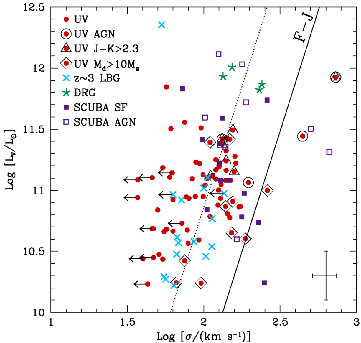
Fig. 9. from The Stellar, Gas, and Dynamical Masses of Starforming Galaxies at z \sim 2 Erb et al. 2006 ApJ 646 107 doi:10.1086/504891 https://dx.doi.org/10.1086/504891 © 2006. The American Astronomical Society. All rights reserved. Printed in U.S.A.
