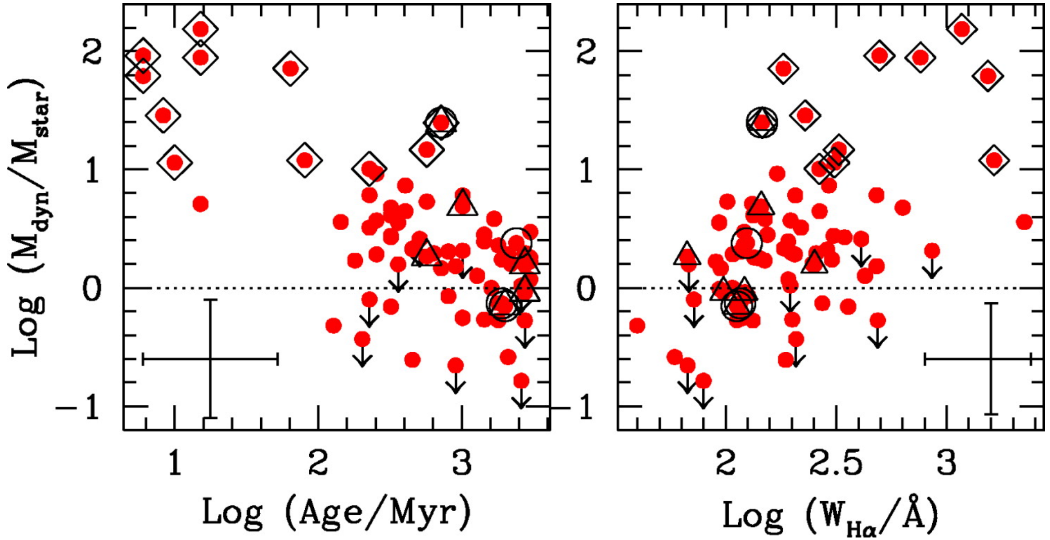
Fig. 8. from The Stellar, Gas, and Dynamical Masses of Starforming Galaxies at z \approx 2 Erb et al. 2006 ApJ 646 107 doi:10.1086/504891 https://dx.doi.org/10.1086/504891 © 2006. The American Astronomical Society. All rights reserved. Printed in U.S.A.
