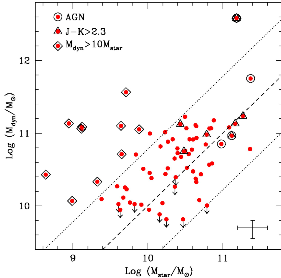
Fig. 7. from The Stellar, Gas, and Dynamical Masses of Starforming Galaxies at z \sim 2 Erb et al. 2006 ApJ 646 107 doi:10.1086/504891 https://dx.doi.org/10.1086/504891 © 2006. The American Astronomical Society. All rights reserved. Printed in U.S.A.
