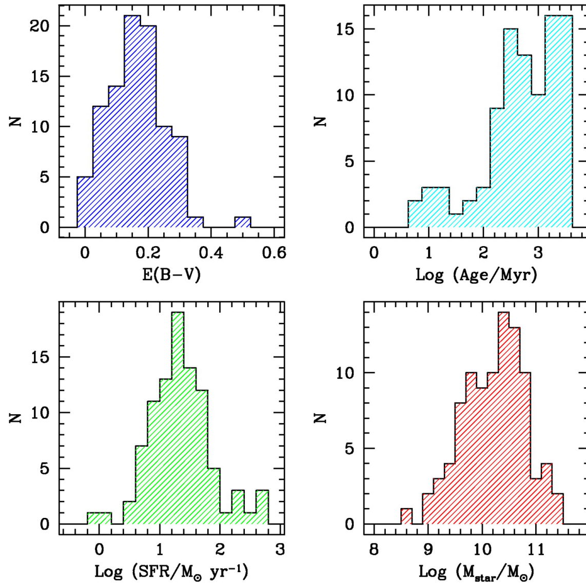
Fig. 5. from The Stellar, Gas, and Dynamical Masses of Starforming Galaxies at z \sim 2 Erb et al. 2006 ApJ 646 107 doi:10.1086/504891 https://dx.doi.org/10.1086/504891 © 2006. The American Astronomical Society. All rights reserved. Printed in U.S.A.
