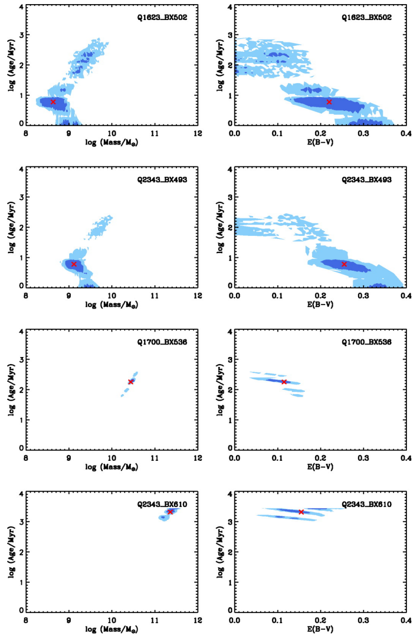
Fig. 4. from The Stellar, Gas, and Dynamical Masses of Starforming Galaxies at z \approx 2 Erb et al. 2006 ApJ 646 107 doi:10.1086/504891 https://dx.doi.org/10.1086/504891
