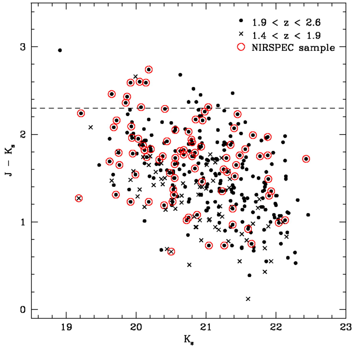
Fig. 1. from The Stellar, Gas, and Dynamical Masses of Starforming Galaxies at z \gtrsim 2 Erb et al. 2006 ApJ 646 107 doi:10.1086/504891 https://dx.doi.org/10.1086/504891 © 2006. The American Astronomical Society. All rights reserved. Printed in U.S.A.
