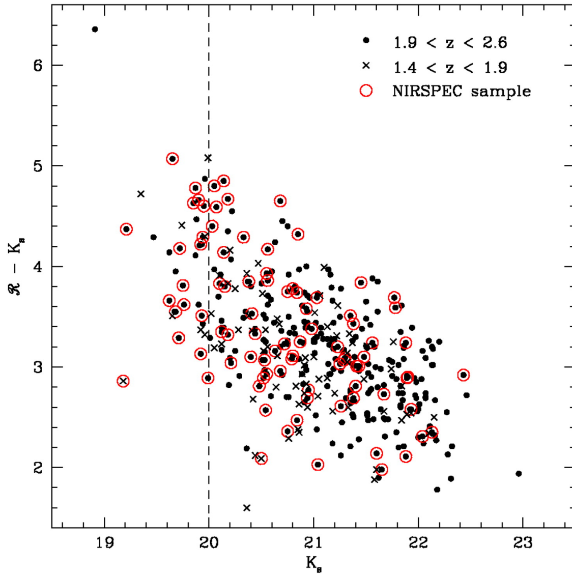
Fig. 1. from The Stellar, Gas, and Dynamical Masses of Starforming Galaxies at z \sim 2 Erb et al. 2006 ApJ 646 107 doi:10.1086/504891 https://dx.doi.org/10.1086/504891 © 2006. The American Astronomical Society. All rights reserved. Printed in U.S.A.
