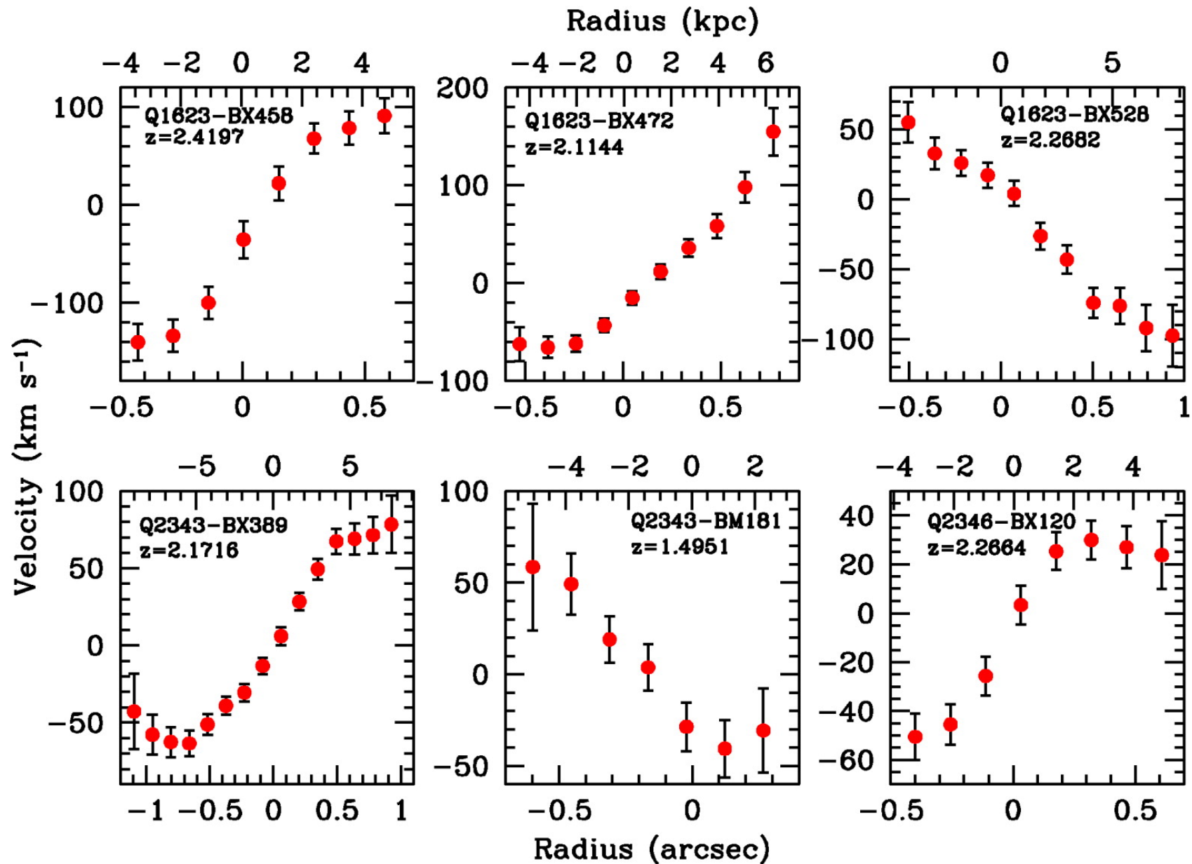
Fig. 14. from The Stellar, Gas, and Dynamical Masses of Starforming Galaxies at z \sim 2 Erb et al. 2006 ApJ 646 107 doi:10.1086/504891 https://dx.doi.org/10.1086/504891 © 2006. The American Astronomical Society. All rights reserved. Printed in U.S.A.
