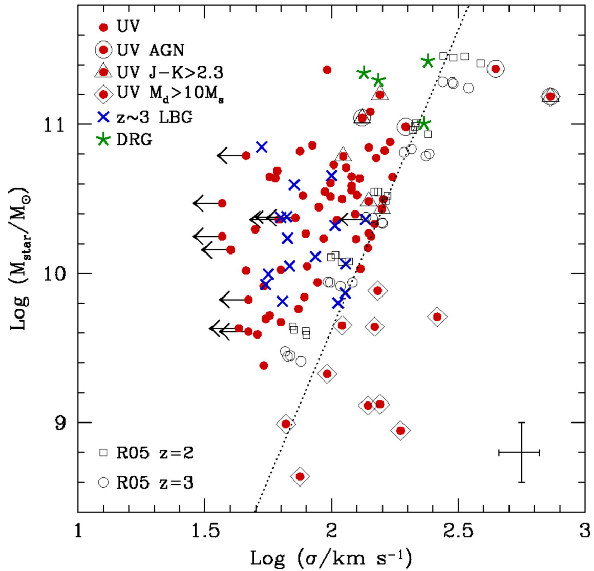
Fig. 12. from The Stellar, Gas, and Dynamical Masses of Starforming Galaxies at z \sim 2 Erb et al. 2006 ApJ 646 107 doi:10.1086/504891 https://dx.doi.org/10.1086/504891 © 2006. The American Astronomical Society. All rights reserved. Printed in U.S.A.
