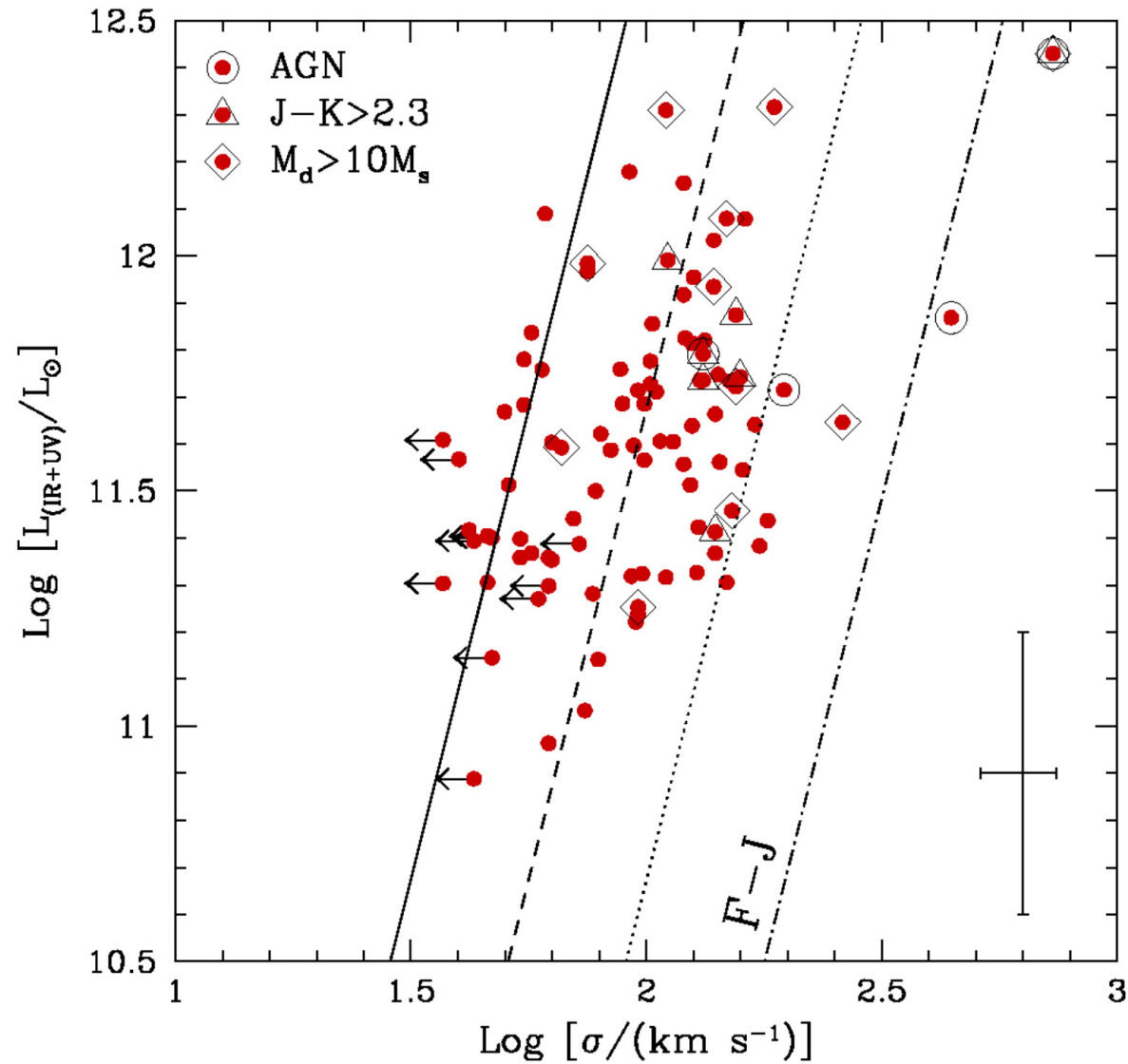
Fig. 11. from The Stellar, Gas, and Dynamical Masses of Starforming Galaxies at z \sim 2 Erb et al. 2006 ApJ 646 107 doi:10.1086/504891 https://dx.doi.org/10.1086/504891 © 2006. The American Astronomical Society. All rights reserved. Printed in U.S.A.
