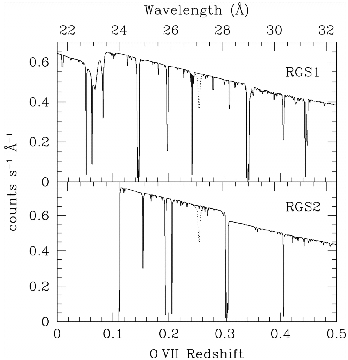
Fig. 2. from XMMNewton View of the z > 0 WarmHot Intergalactic Medium toward Markarian 421 Williams et al. 2006 ApJL 642 L95 doi:10.1086/504635 https://dx.doi.org/10.1086/504635
