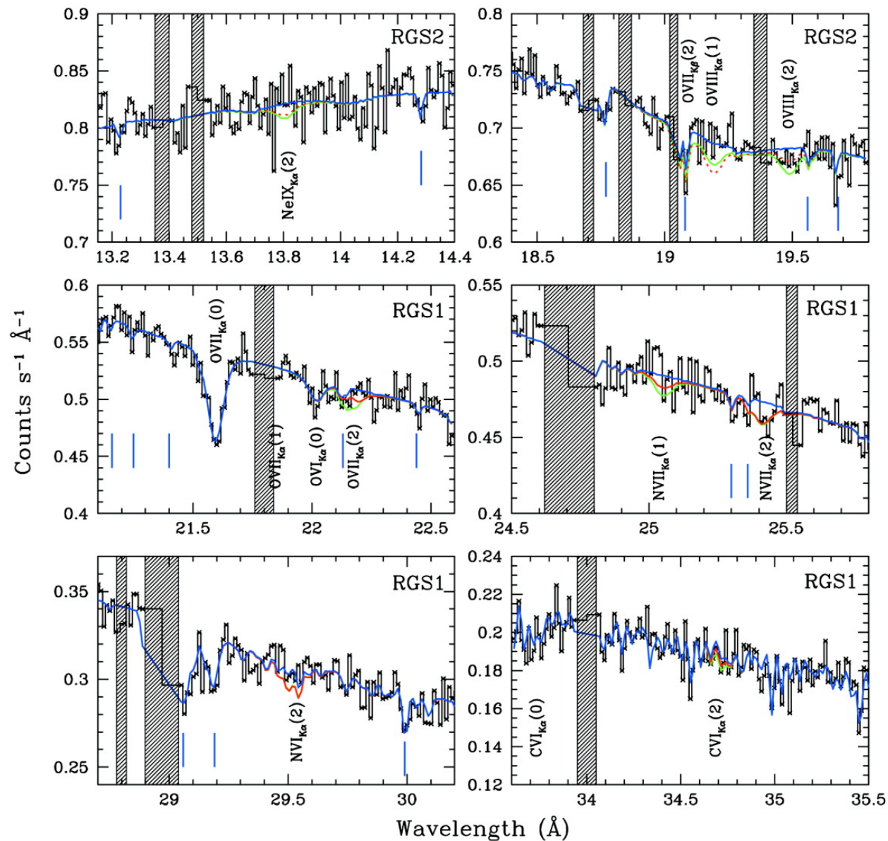
Fig. 1. from XMMNewton View of the z > 0 WarmHot Intergalactic Medium toward Markarian 421 Williams et al. 2006 ApJL 642 L95 doi:10.1086/504635 https://dx.doi.org/10.1086/504635 © 2006. The American Astronomical Society. All rights reserved. Printed in U.S.A.
