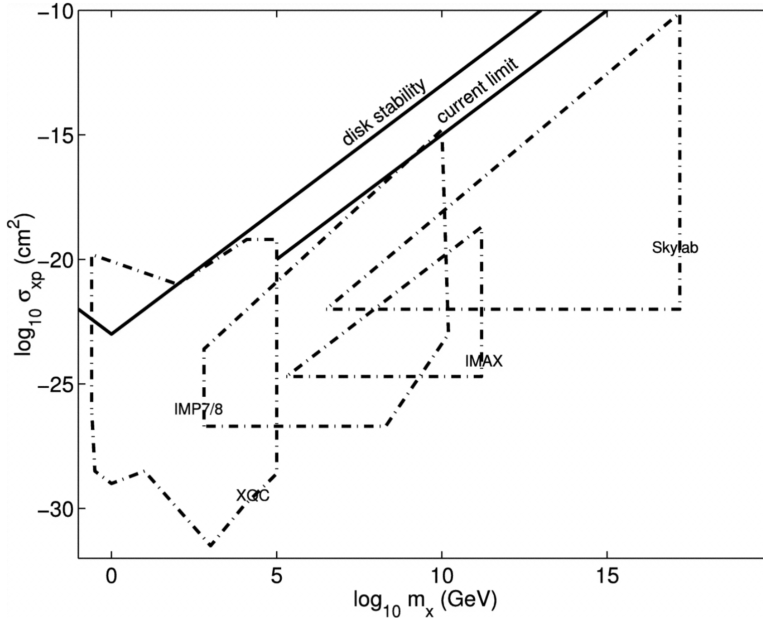
Fig. 4. from Consequences of ShortRange Interactions between Dark Matter and Protons in Galaxy Clusters Chuzhoy & Nusser 2006 ApJ 645 950 doi:10.1086/504505 https://dx.doi.org/10.1086/504505 © 2006. The American Astronomical Society. All rights reserved. Printed in U.S.A.
