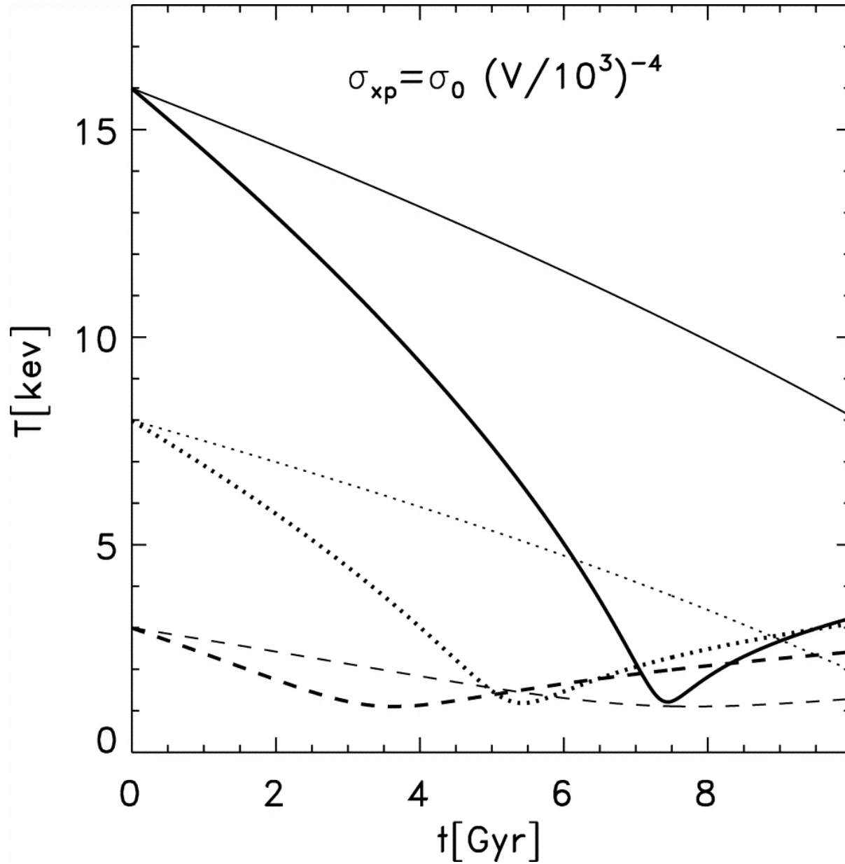
Fig. 3. from Consequences of ShortRange Interactions between Dark Matter and Protons in Galaxy Clusters Chuzhoy & Nusser 2006 ApJ 645 950 doi:10.1086/504505 https://dx.doi.org/10.1086/504505 © 2006. The American Astronomical Society. All rights reserved. Printed in U.S.A.
