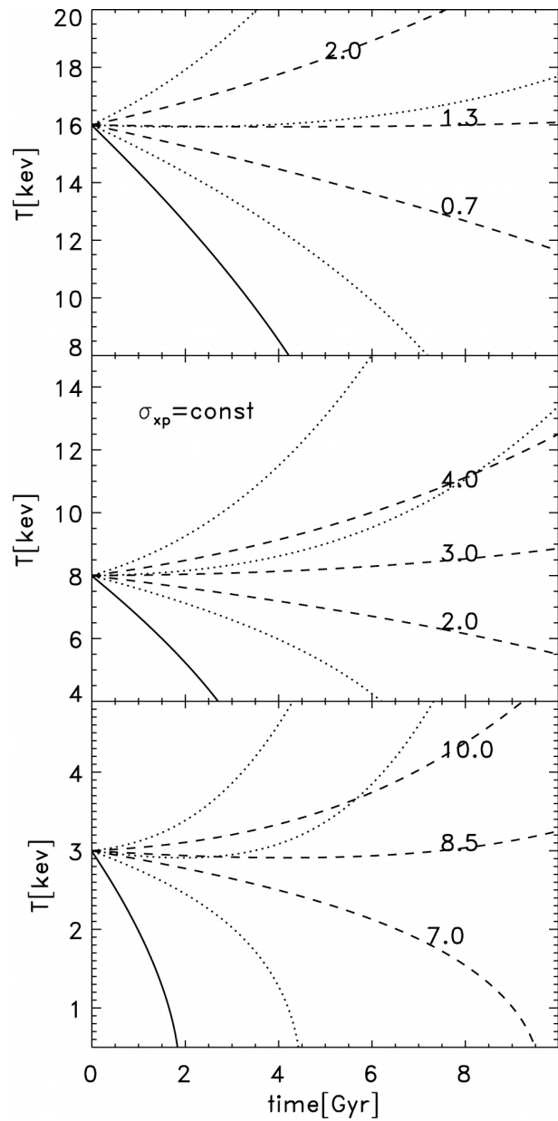
Fig. 2. from Consequences of ShortRange Interactions between Dark Matter and Protons in Galaxy Clusters Chuzhoy & Nusser 2006 ApJ 645 950 doi:10.1086/504505 https://dx.doi.org/10.1086/504505
