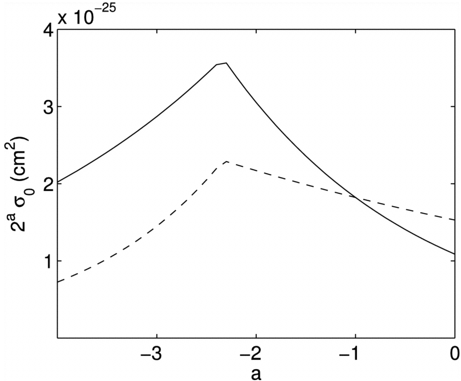
Fig. 1. from Consequences of ShortRange Interactions between Dark Matter and Protons in Galaxy Clusters Chuzhoy & Nusser 2006 ApJ 645 950 doi:10.1086/504505 https://dx.doi.org/10.1086/504505 © 2006. The American Astronomical Society. All rights reserved. Printed in U.S.A.
