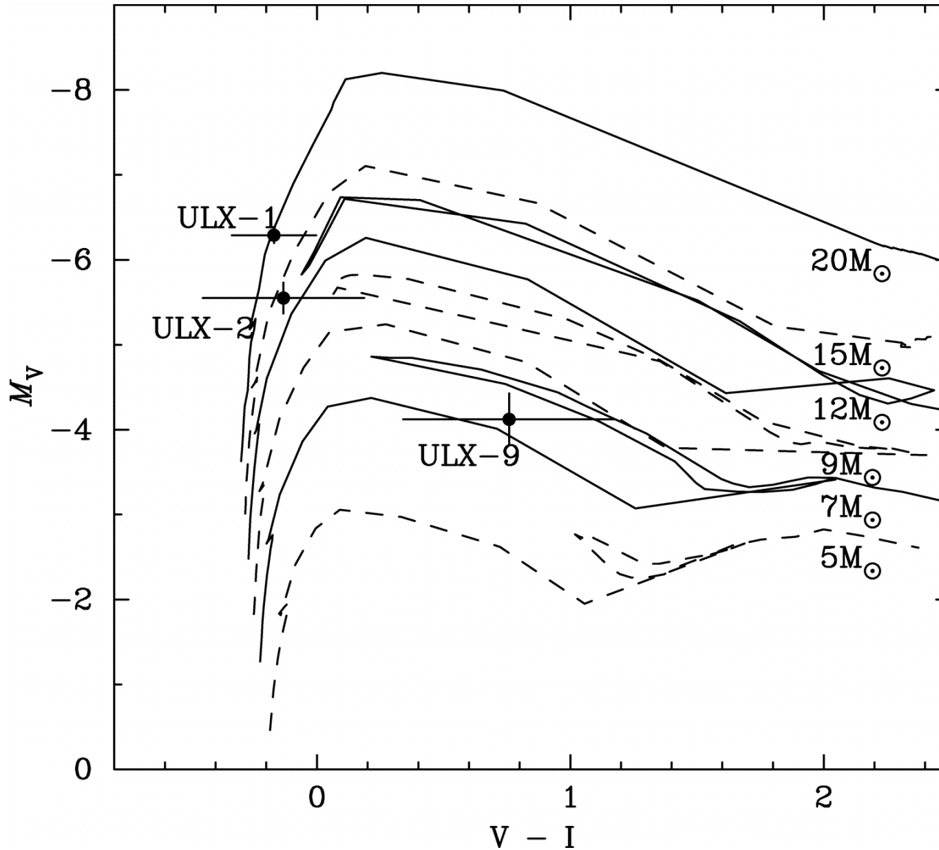
Fig. 4. from Hubble Space Telescope Identification of the Optical Counterparts of Ultraluminous XRay Sources in M51 Terashima, Inoue, & Wilson 2006 ApJ 645 264 doi:10.1086/504251 https://dx.doi.org/10.1086/504251 © 2006. The American Astronomical Society. All rights reserved. Printed in U.S.A.
