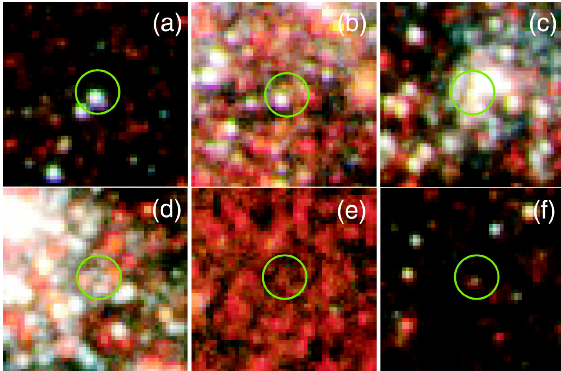
Fig. 3. from Hubble Space Telescope Identification of the Optical Counterparts of Ultraluminous XRay Sources in M51 Terashima, Inoue, & Wilson 2006 ApJ 645 264 doi:10.1086/504251 https://dx.doi.org/10.1086/504251 © 2006. The American Astronomical Society. All rights reserved. Printed in U.S.A.
