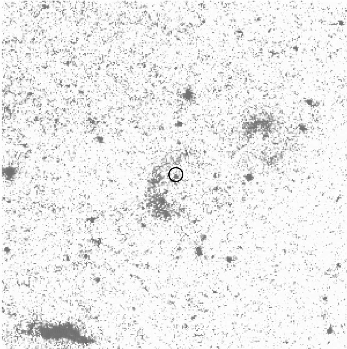
Fig. 2. from Hubble Space Telescope Identification of the Optical Counterparts of Ultraluminous XRay Sources in M51 Terashima, Inoue, & Wilson 2006 ApJ 645 264 doi:10.1086/504251 https://dx.doi.org/10.1086/504251 © 2006. The American Astronomical Society. All rights reserved. Printed in U.S.A.
