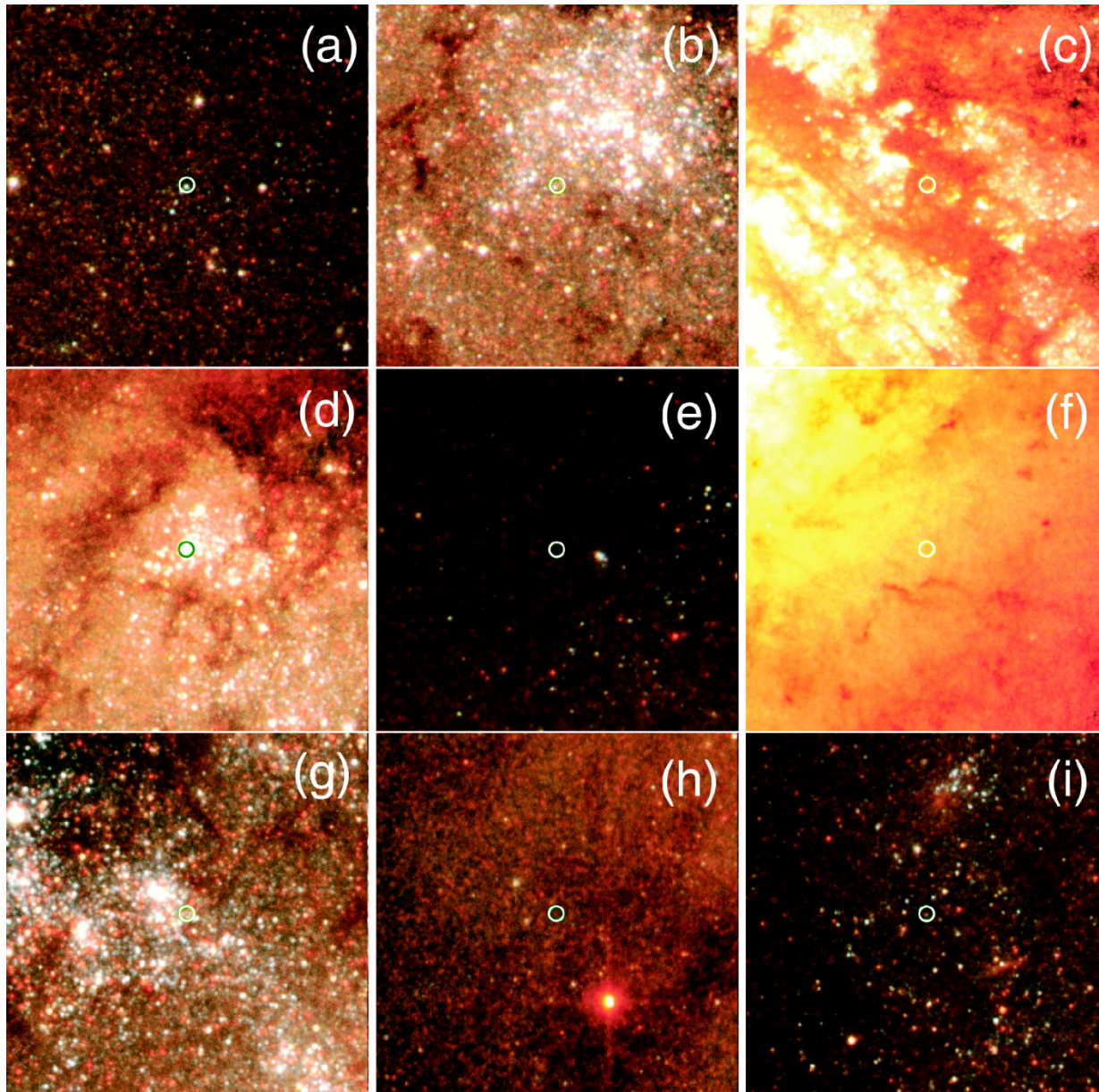
Fig. 1. from Hubble Space Telescope Identification of the Optical Counterparts of Ultraluminous XRay Sources in M51 Terashima, Inoue, & Wilson 2006 ApJ 645 264 doi:10.1086/504251 https://dx.doi.org/10.1086/504251 © 2006. The American Astronomical Society. All rights reserved. Printed in U.S.A.
