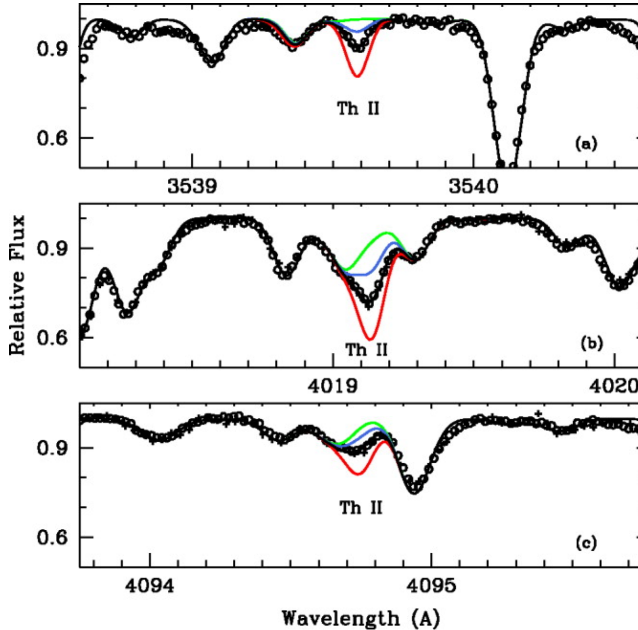
Fig. 7. from NearUltraviolet Observations of HD 221170: New Insights into the Nature of rProcess-rich Stars Ivans et al. 2006 ApJ 645 613 doi:10.1086/504069 https://dx.doi.org/10.1086/504069 © 2006. The American Astronomical Society. All rights reserved. Printed in U.S.A.
