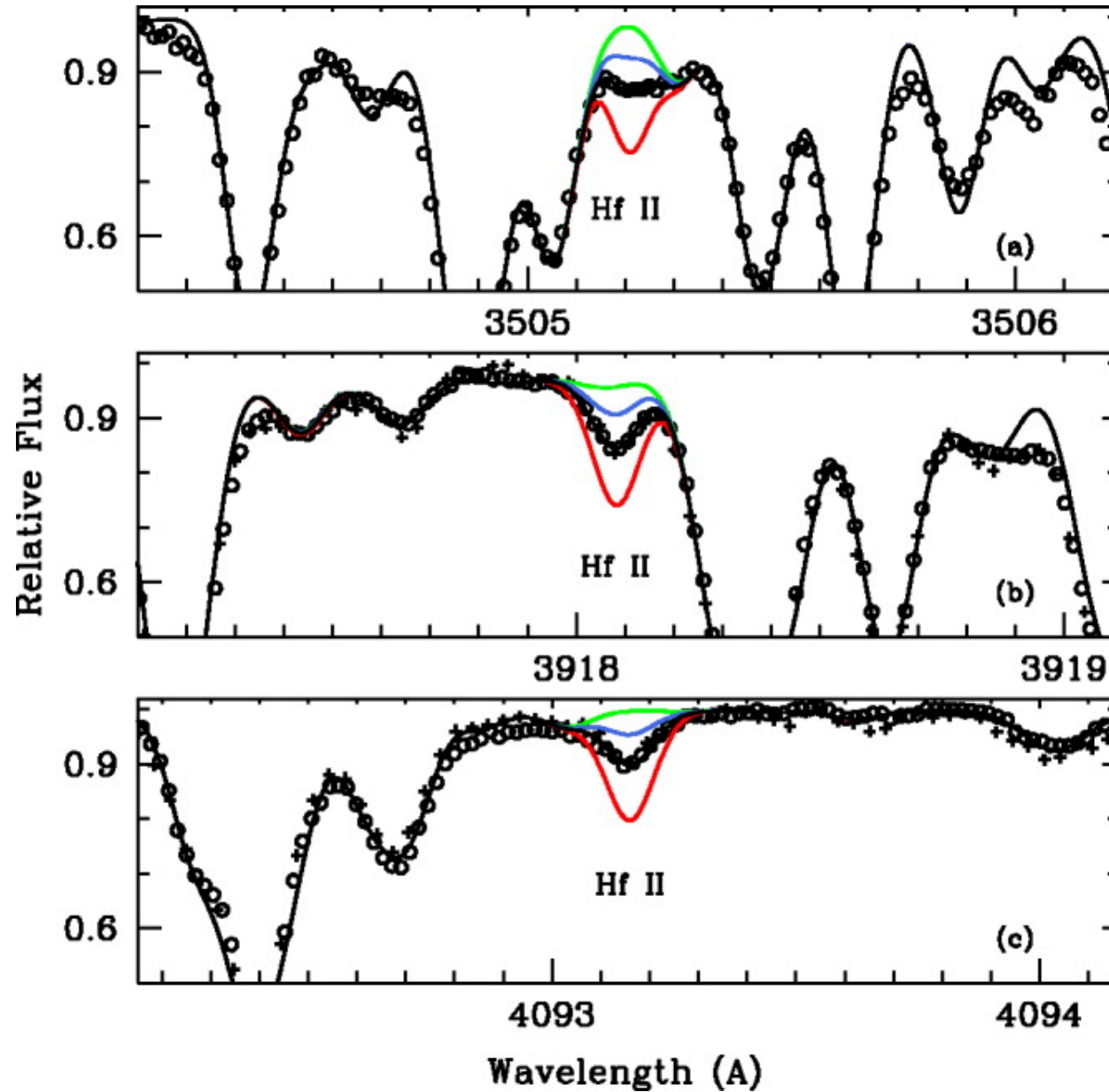
Fig. 6. from NearUltraviolet Observations of HD 221170: New Insights into the Nature of rProcess-rich Stars Ivans et al. 2006 ApJ 645 613 doi:10.1086/504069 https://dx.doi.org/10.1086/504069 © 2006. The American Astronomical Society. All rights reserved. Printed in U.S.A.
