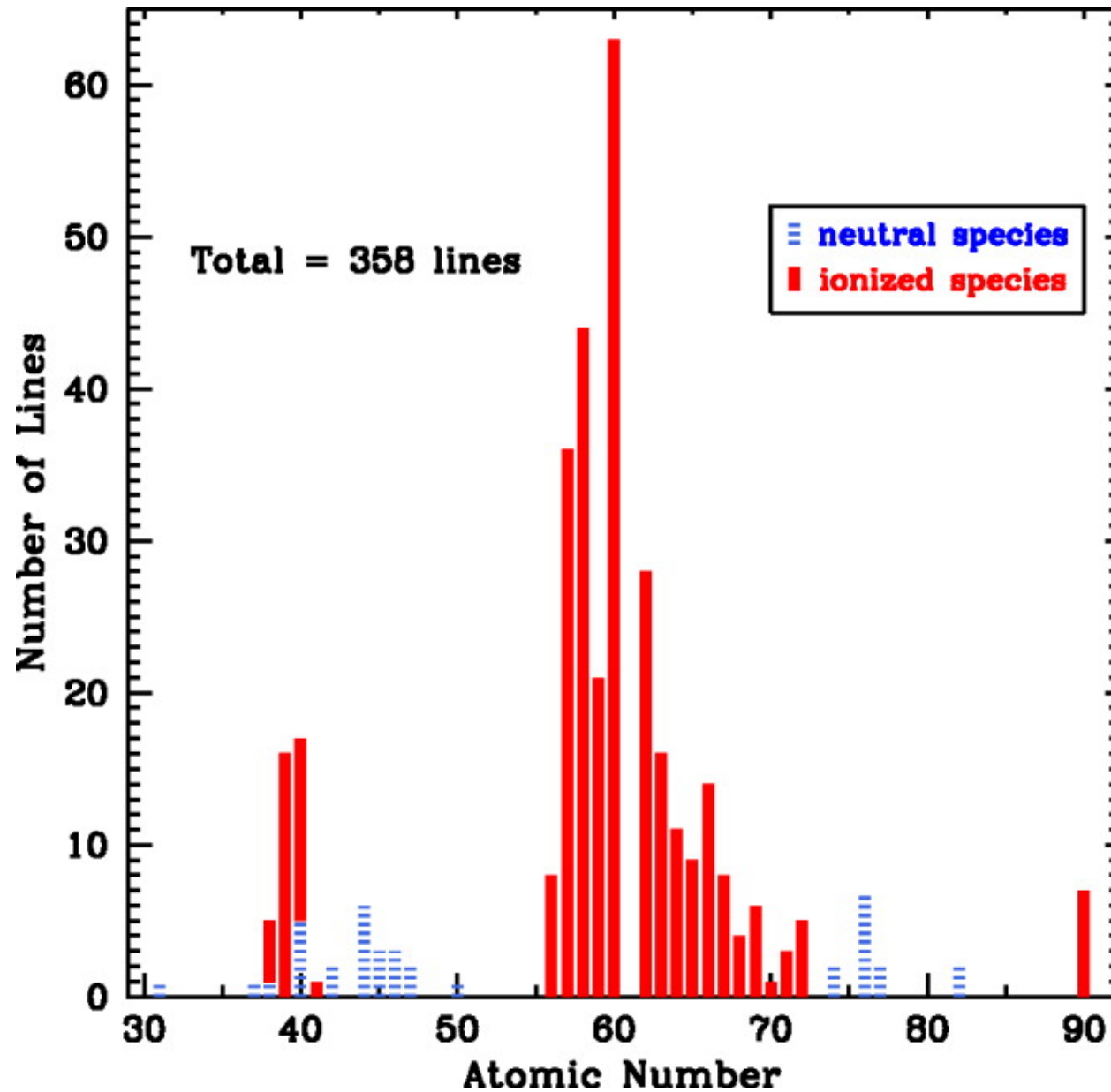
Fig. 3. from NearUltraviolet Observations of HD 221170: New Insights into the Nature of rProcess-rich Stars Ivans et al. 2006 ApJ 645 613 doi:10.1086/504069 https://dx.doi.org/10.1086/504069 © 2006. The American Astronomical Society. All rights reserved. Printed in U.S.A.
