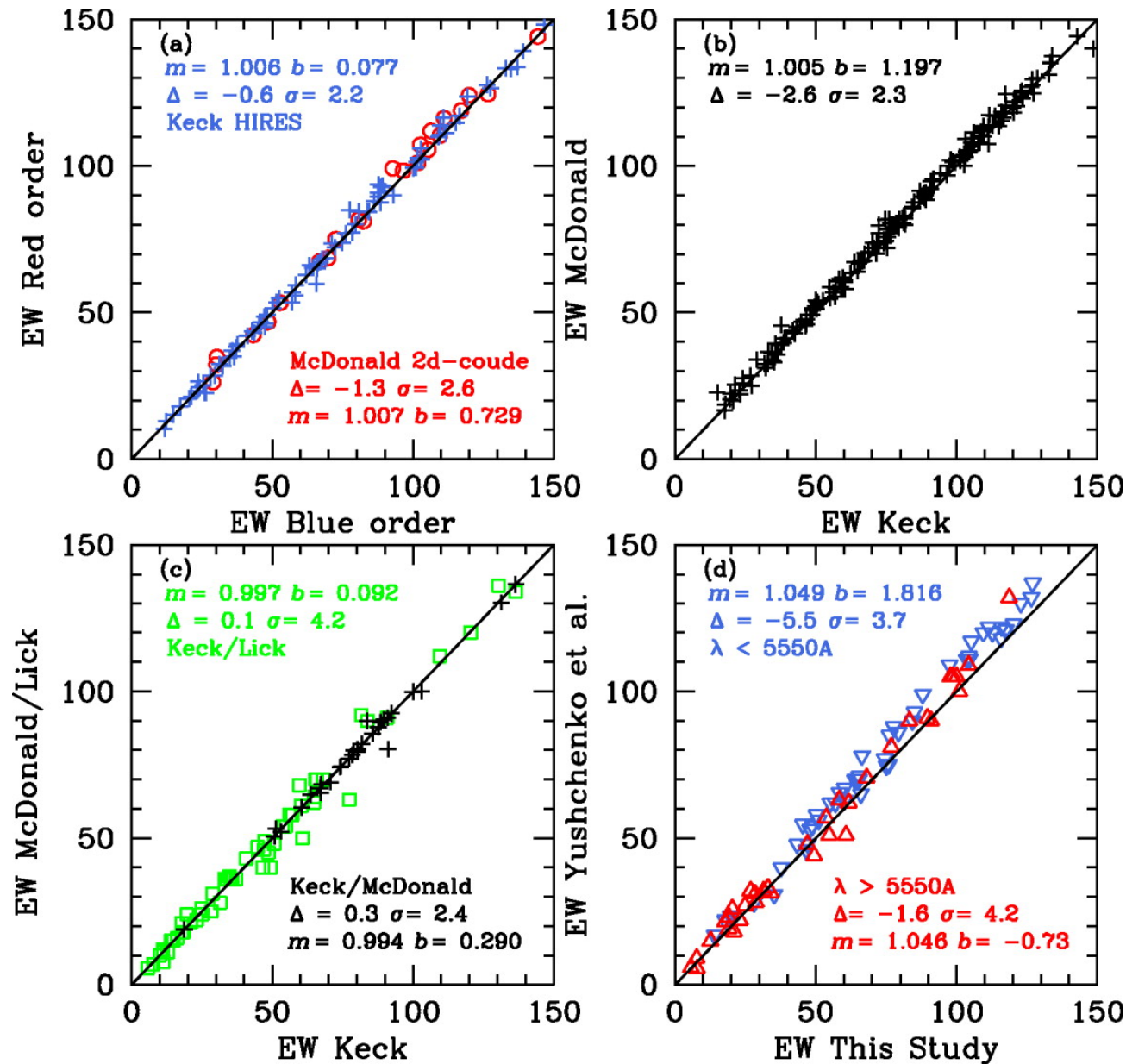
Fig. 2. from NearUltraviolet Observations of HD 221170: New Insights into the Nature of rProcess–rich Stars Ivans et al. 2006 ApJ 645 613 doi:10.1086/504069 https://dx.doi.org/10.1086/504069
