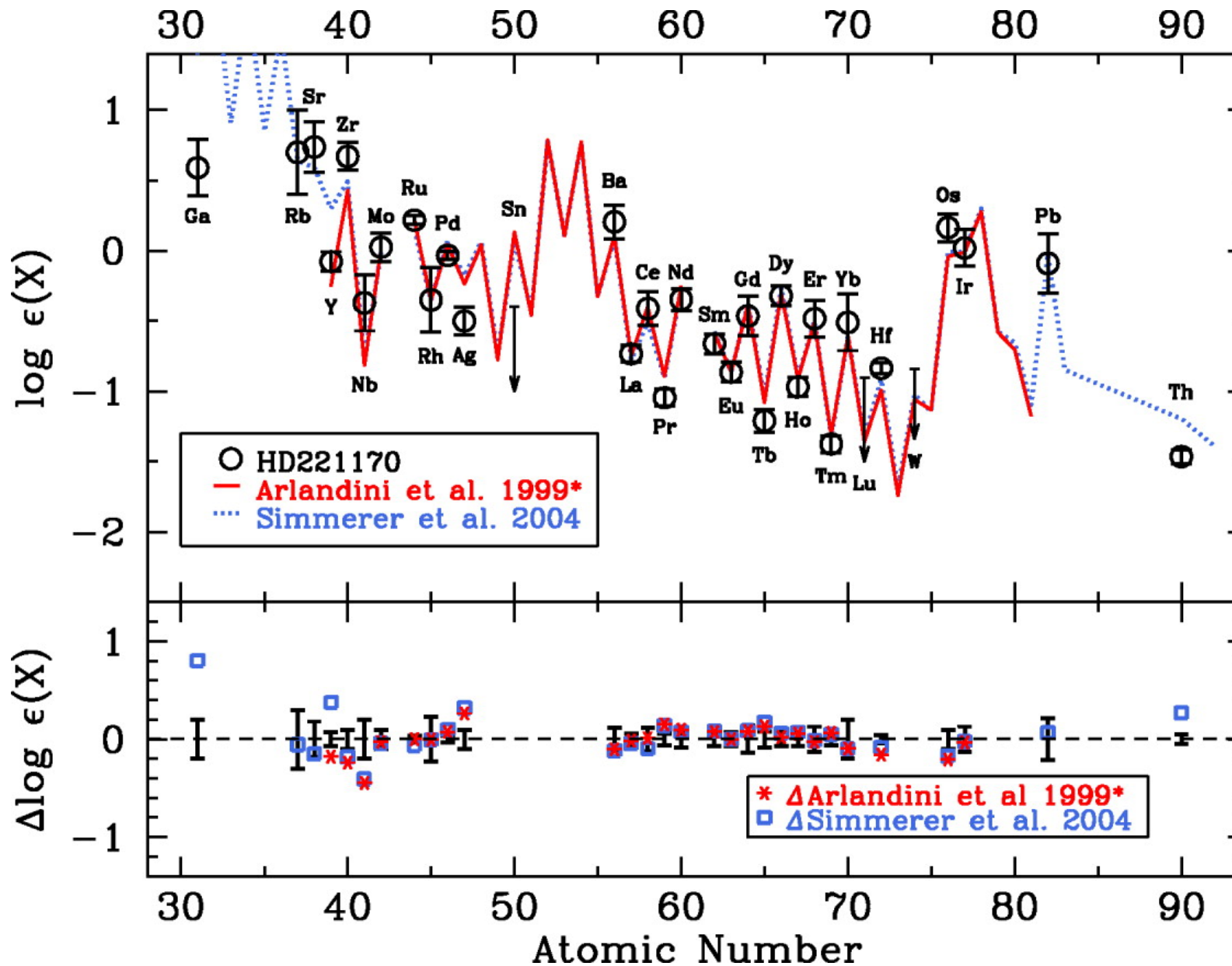
Fig. 10. from NearUltraviolet Observations of HD 221170: New Insights into the Nature of rProcess-rich Stars Ivans et al. 2006 ApJ 645 613 doi:10.1086/504069 https://dx.doi.org/10.1086/504069 © 2006. The American Astronomical Society. All rights reserved. Printed in U.S.A.
