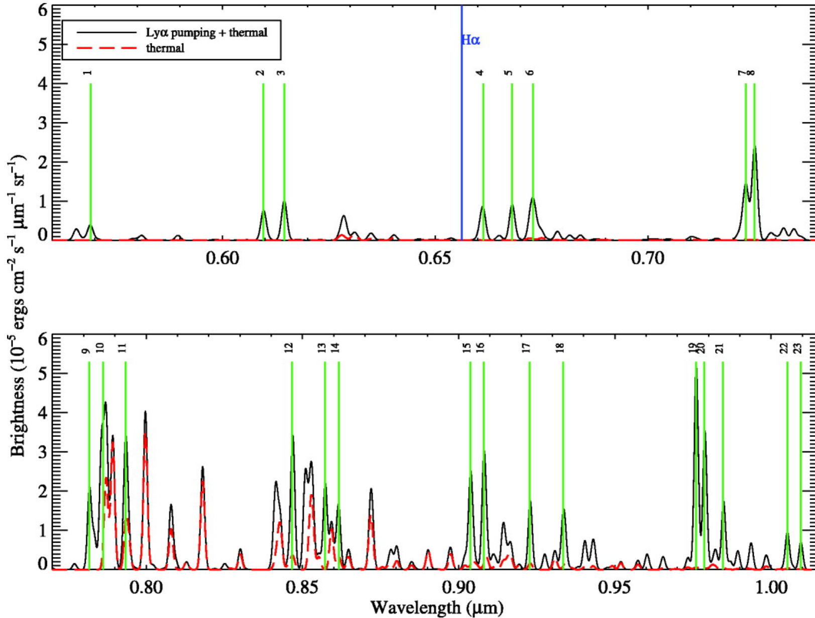
Fig. 6. from Discovery of Lypumped Molecular Hydrogen Emission in the Planetary Nebulae NGC 6853 and NGC 3132 Lupu, France, & McCandliss 2006 ApJ 644 981 doi:10.1086/503603 https://dx.doi.org/10.1086/503603
