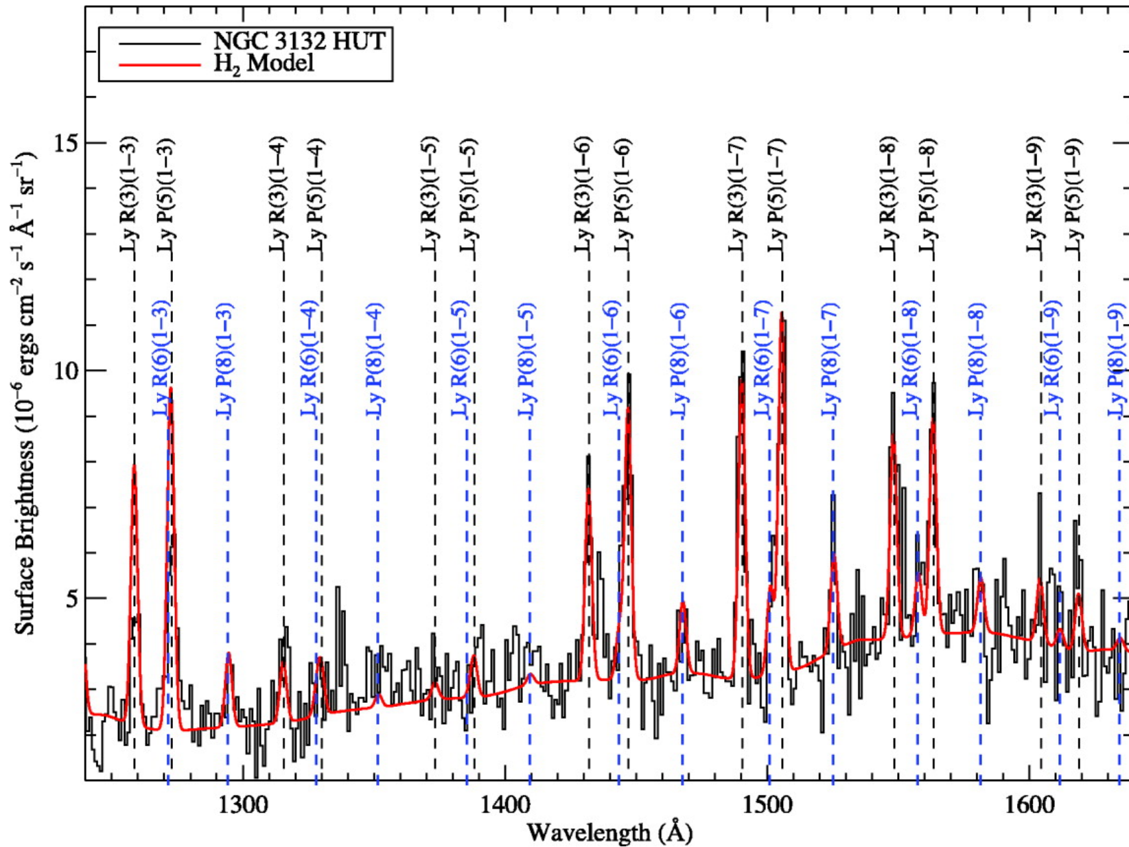
Fig. 5. from Discovery of Lypumped Molecular Hydrogen Emission in the Planetary Nebulae NGC 6853 and NGC 3132 Lupu, France, & McCandliss 2006 ApJ 644 981 doi:10.1086/503603 https://dx.doi.org/10.1086/503603 © 2006. The American Astronomical Society. All rights reserved. Printed in U.S.A.
