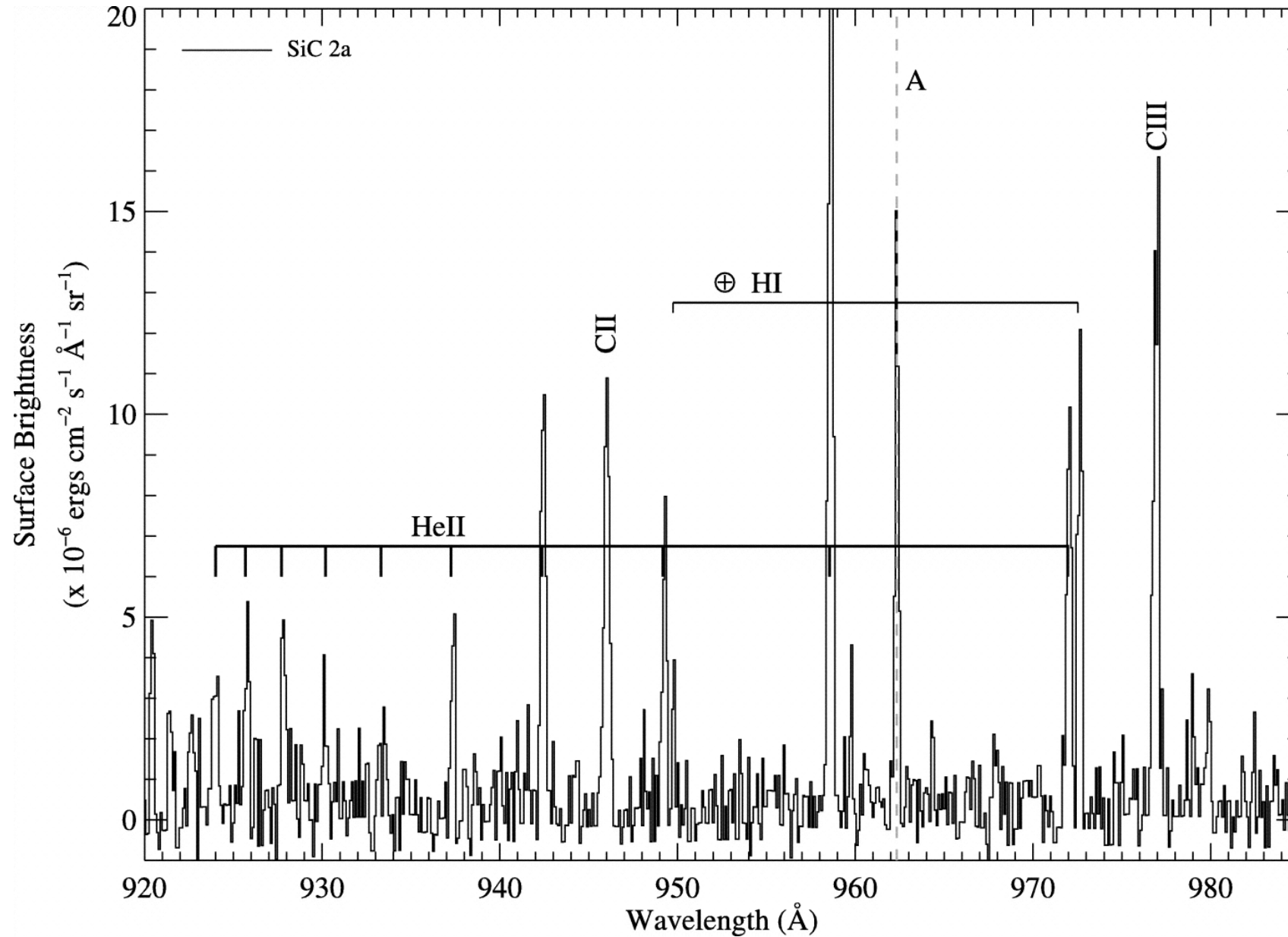
Fig. 3. from Discovery of Lypumped Molecular Hydrogen Emission in the Planetary Nebulae NGC 6853 and NGC 3132 Lupu, France, & McCandliss 2006 ApJ 644 981 doi:10.1086/503603 https://dx.doi.org/10.1086/503603
