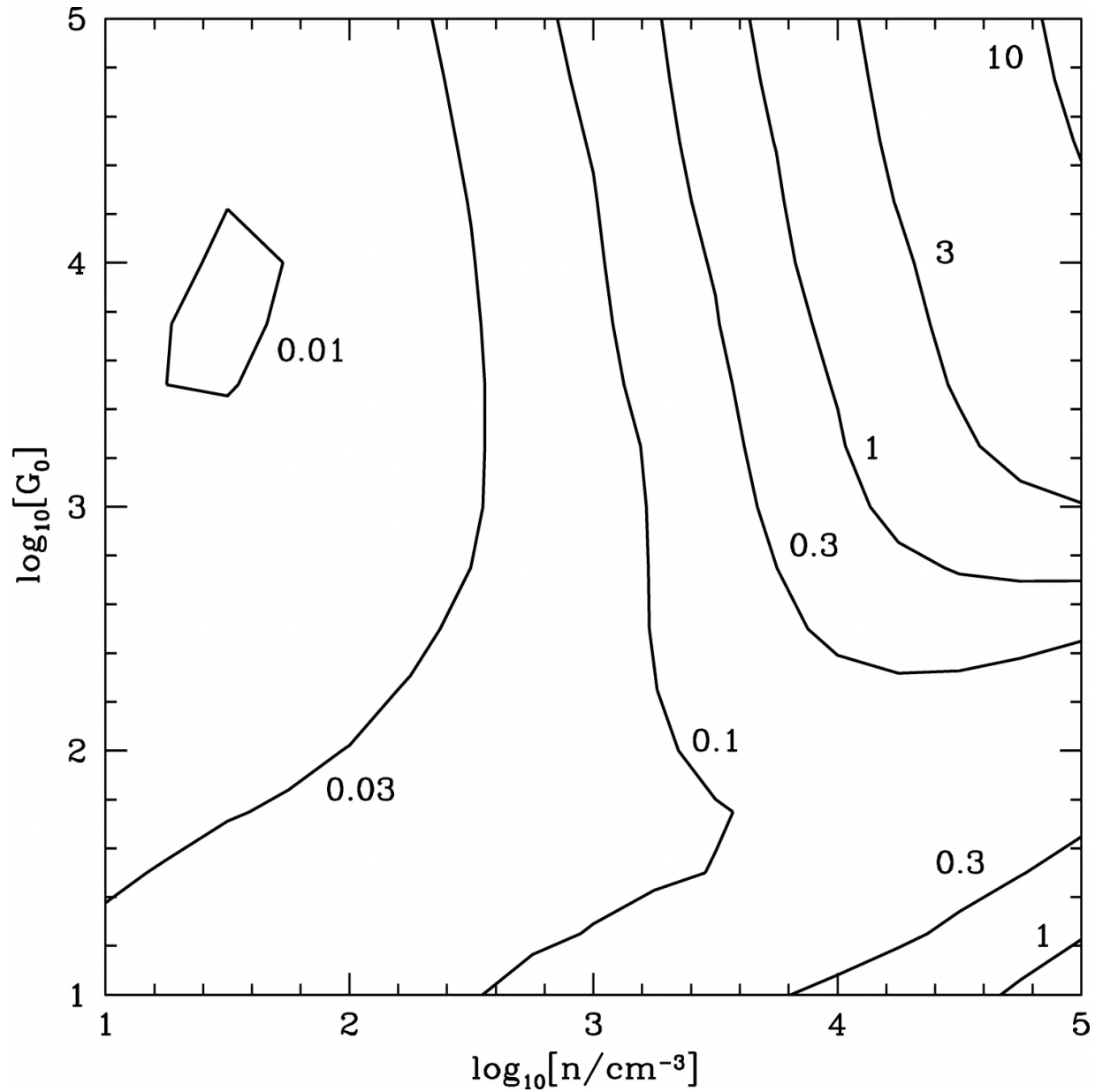
Fig. 9. from [Si II], [Fe II], [C II], and H2 Emission from Massive Starforming Regions Kaufman, Wolfire, & Hollenbach 2006 ApJ 644 283 doi:10.1086/503596 https://dx.doi.org/10.1086/503596
