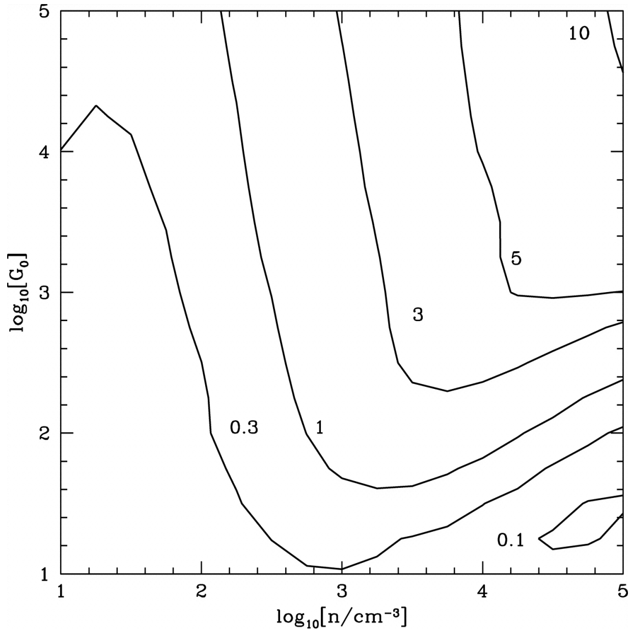
Fig. 8. from [Si II], [Fe II], [C II], and H2 Emission from Massive Starforming Regions Kaufman, Wolfire, & Hollenbach 2006 ApJ 644 283 doi:10.1086/503596 https://dx.doi.org/10.1086/503596
