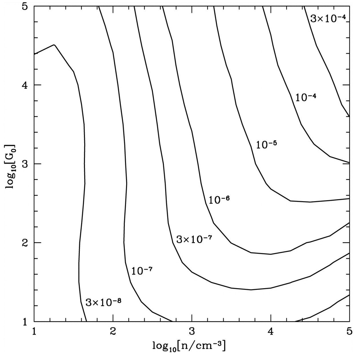
Fig. 6. from [Si II], [Fe II], [C II], and H 2 Emission from Massive Starforming Regions Kaufman, Wolfire, & Hollenbach 2006 ApJ 644 283 doi:10.1086/503596 https://dx.doi.org/10.1086/503596
