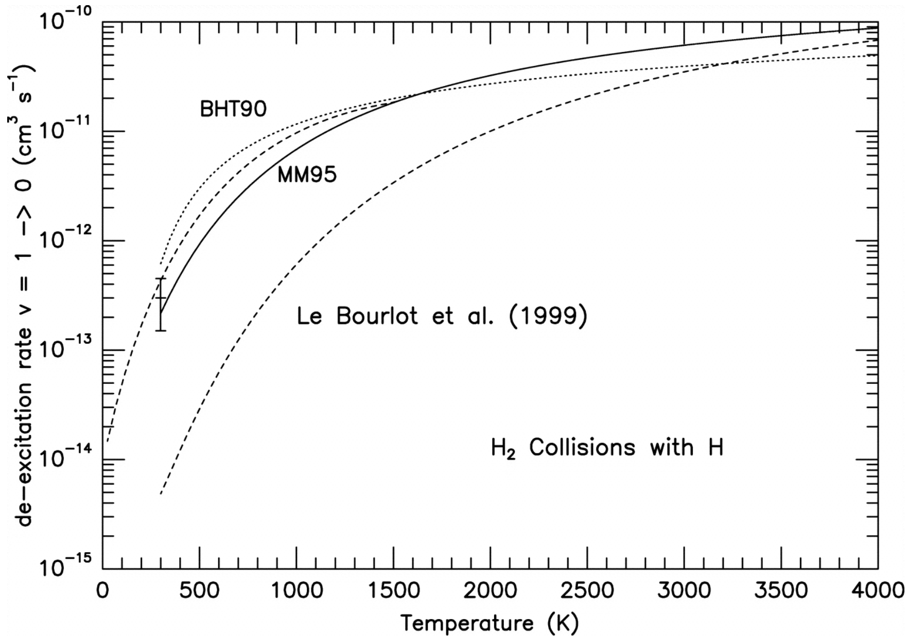
Fig. 3. from [Si II], [Fe II], [C II], and H 2 Emission from Massive Starforming Regions Kaufman, Wolfire, & Hollenbach 2006 ApJ 644 283 doi:10.1086/503596 https://dx.doi.org/10.1086/503596
