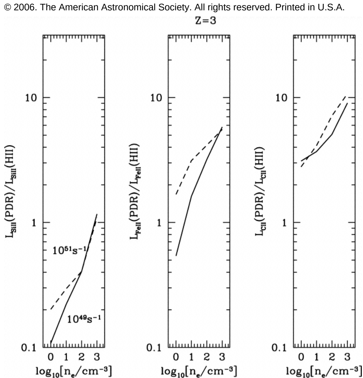
Fig. 21. from [Si II], [Fe II], [C II], and H2 Emission from Massive Starforming Regions Kaufman, Wolfire, & Hollenbach 2006 ApJ 644 283 doi:10.1086/503596 https://dx.doi.org/10.1086/503596
