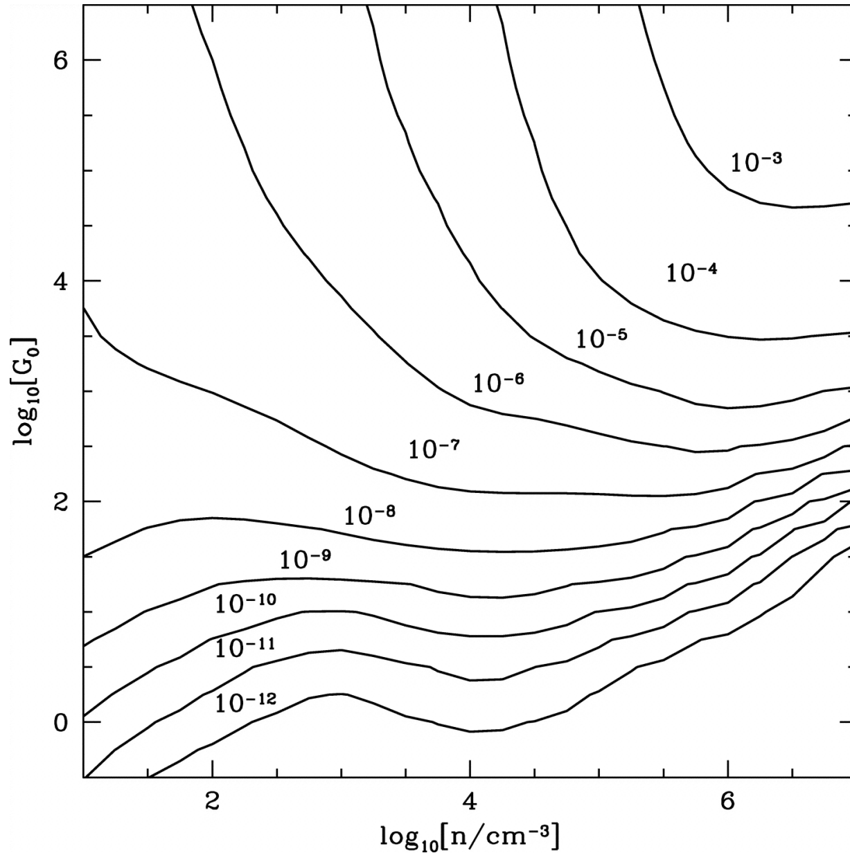
Fig. 2. from [Si II], [Fe II], [C II], and H2 Emission from Massive Starforming Regions Kaufman, Wolfire, & Hollenbach 2006 ApJ 644 283 doi:10.1086/503596 https://dx.doi.org/10.1086/503596
