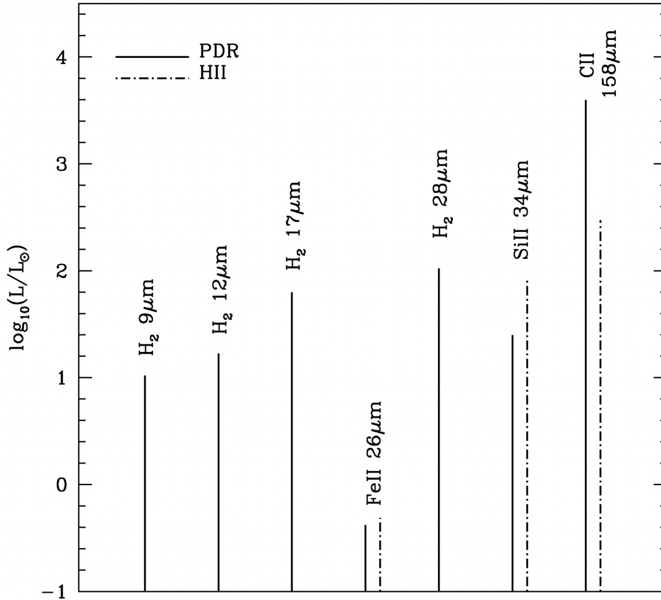
Fig. 19. from [Si II], [Fe II], [C II], and H 2 Emission from Massive Starforming Regions Kaufman, Wolfire, & Hollenbach 2006 ApJ 644 283 doi:10.1086/503596 https://dx.doi.org/10.1086/503596 © 2006. The American Astronomical Society. All rights reserved. Printed in U.S.A.
