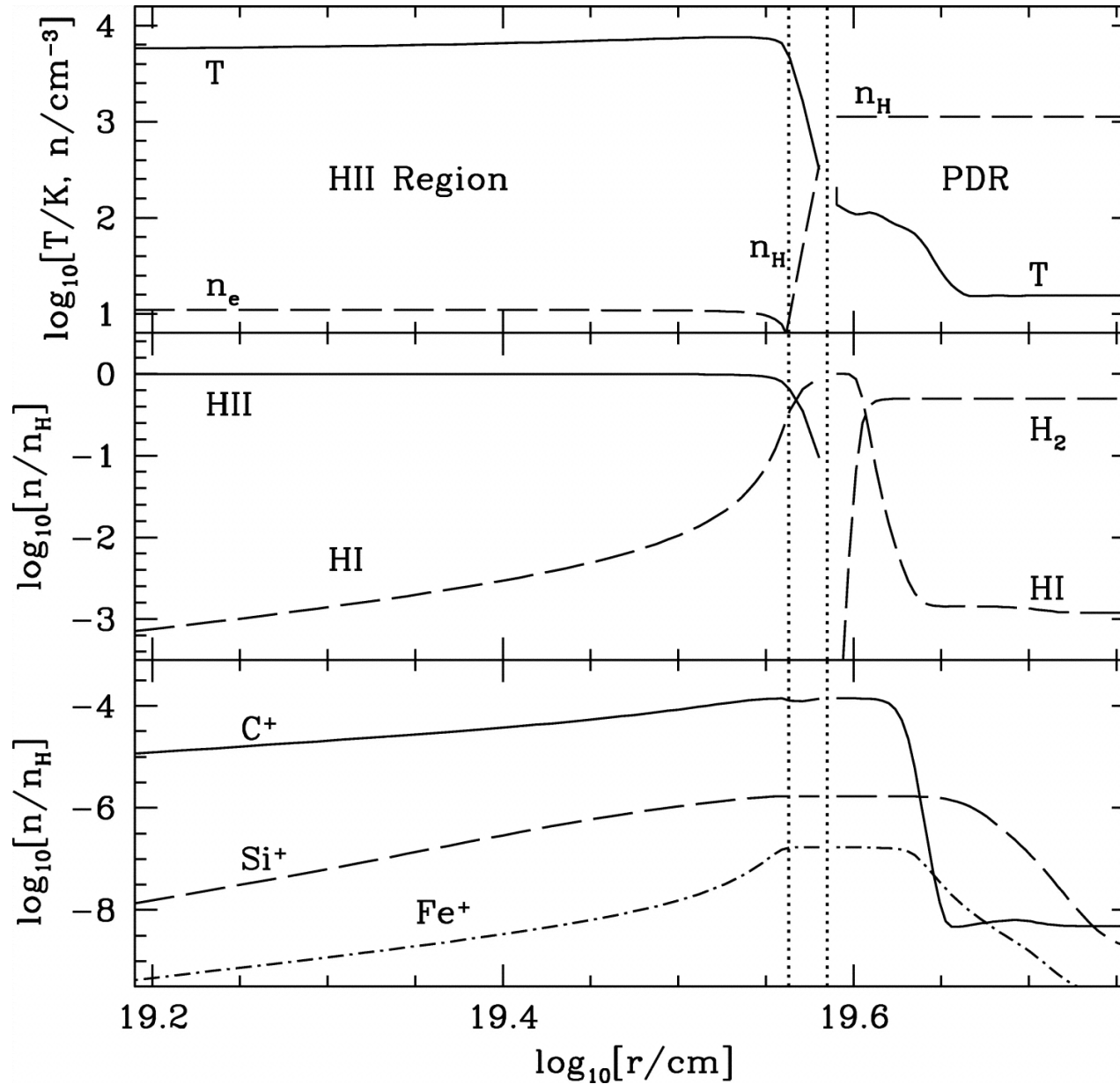
Fig. 18. from [Si II], [Fe II], [C II], and H 2 Emission from Massive Starforming Regions Kaufman, Wolfire, & Hollenbach 2006 ApJ 644 283 doi:10.1086/503596 https://dx.doi.org/10.1086/503596
