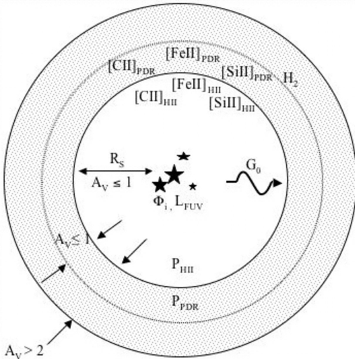
Fig. 16. from [Si II], [Fe II], [C II], and H 2 Emission from Massive Starforming Regions Kaufman, Wolfire, & Hollenbach 2006 ApJ 644 283 doi:10.1086/503596 https://dx.doi.org/10.1086/503596 © 2006. The American Astronomical Society. All rights reserved. Printed in U.S.A.
