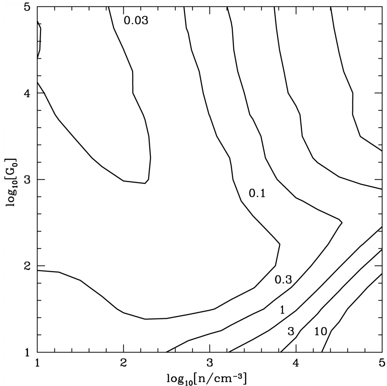
Fig. 15. from [Si II], [Fe II], [C II], and H 2 Emission from Massive Starforming Regions Kaufman, Wolfire, & Hollenbach 2006 ApJ 644 283 doi:10.1086/503596 https://dx.doi.org/10.1086/503596
