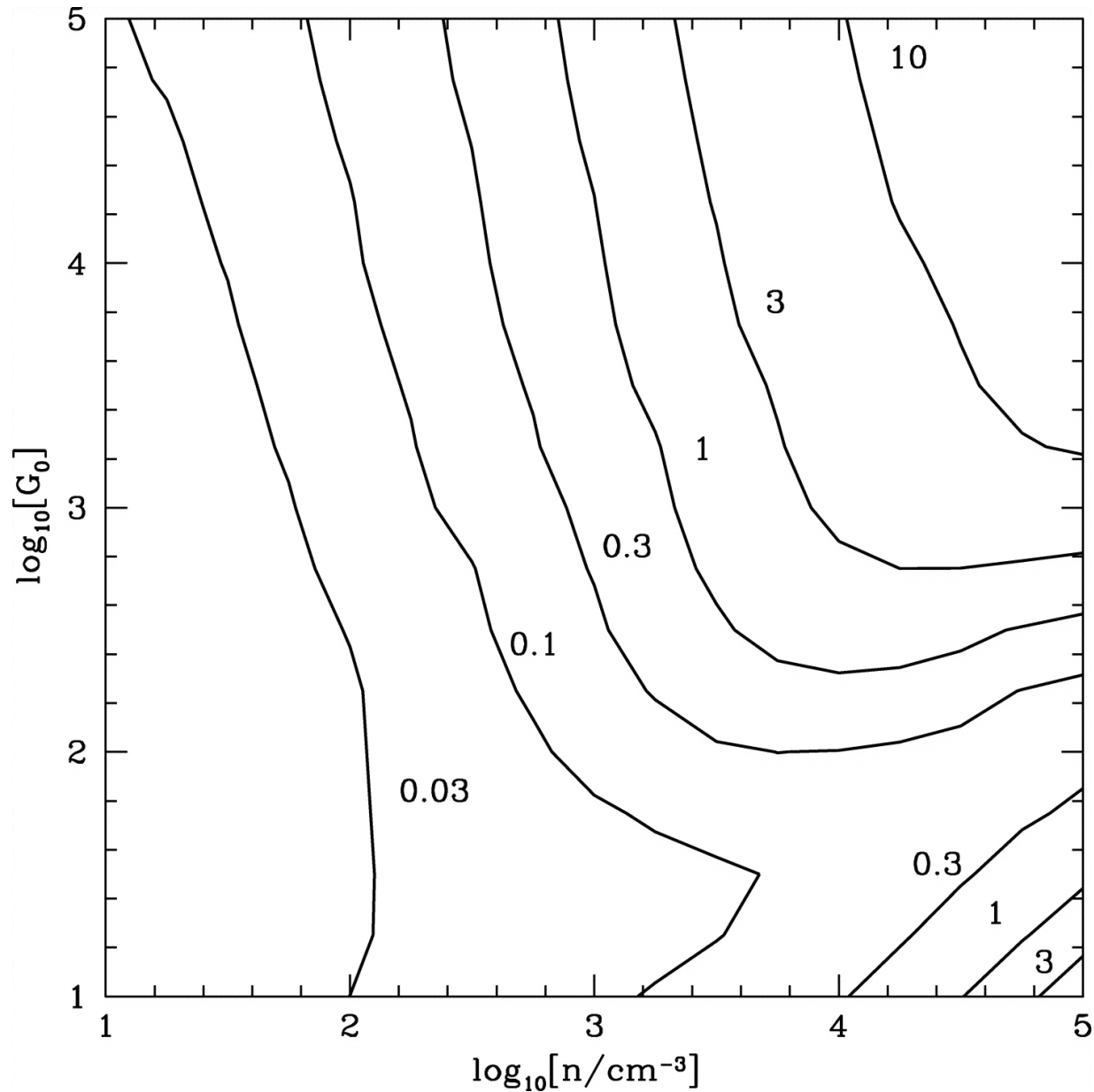
Fig. 14. from [Si II], [Fe II], [C II], and H 2 Emission from Massive Starforming Regions Kaufman, Wolfire, & Hollenbach 2006 ApJ 644 283 doi:10.1086/503596 https://dx.doi.org/10.1086/503596
