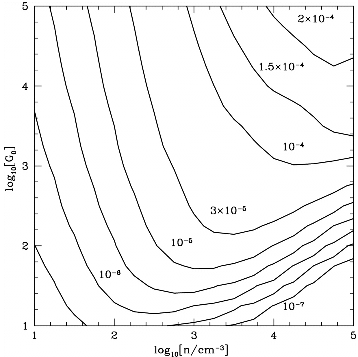
Fig. 13. from [Si II], [Fe II], [C II], and H 2 Emission from Massive Starforming Regions Kaufman, Wolfire, & Hollenbach 2006 ApJ 644 283 doi:10.1086/503596 https://dx.doi.org/10.1086/503596
