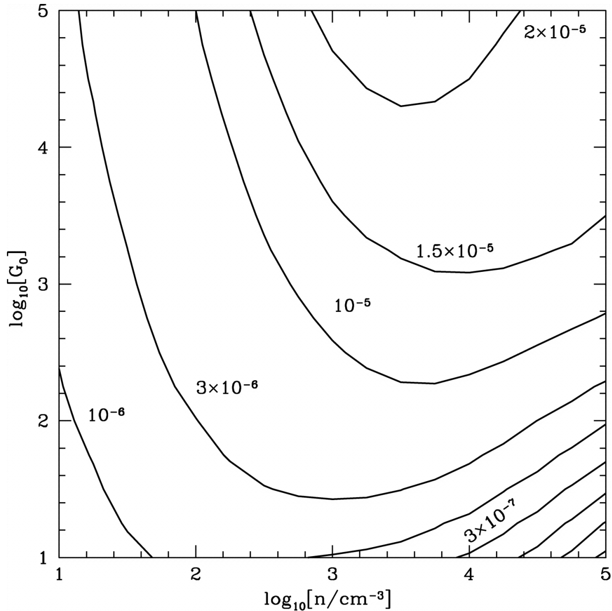
Fig. 12. from [Si II], [Fe II], [C II], and H 2 Emission from Massive Starforming Regions Kaufman, Wolfire, & Hollenbach 2006 ApJ 644 283 doi:10.1086/503596 https://dx.doi.org/10.1086/503596
