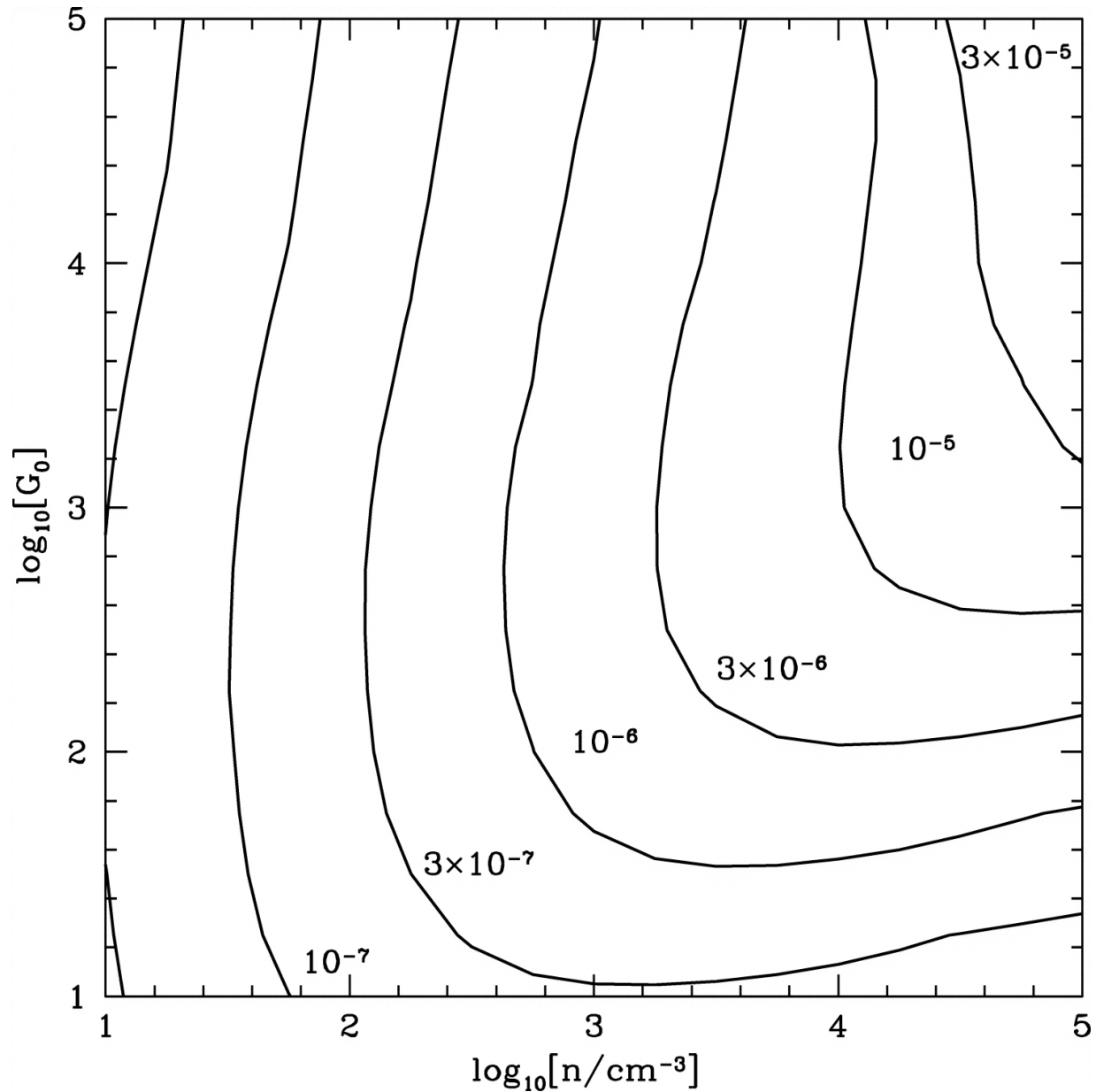
Fig. 11. from [Si II], [Fe II], [C II], and H2 Emission from Massive Starforming Regions Kaufman, Wolfire, & Hollenbach 2006 ApJ 644 283 doi:10.1086/503596 https://dx.doi.org/10.1086/503596
