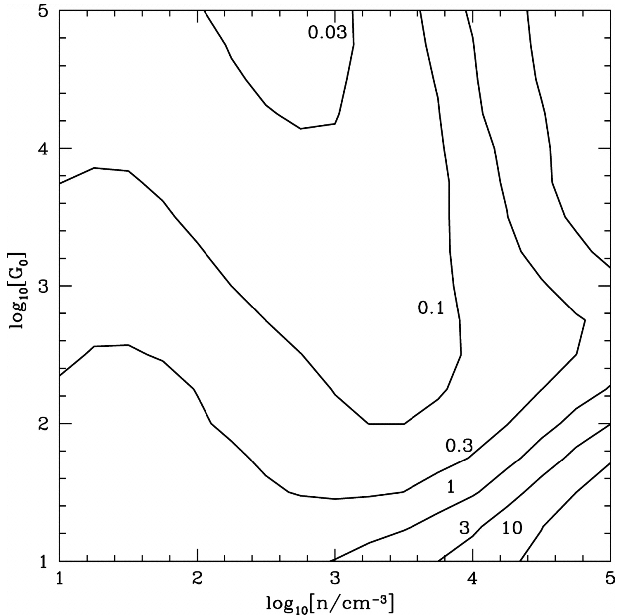
Fig. 10. from [Si II], [Fe II], [C II], and H 2 Emission from Massive Starforming Regions Kaufman, Wolfire, & Hollenbach 2006 ApJ 644 283 doi:10.1086/503596 https://dx.doi.org/10.1086/503596
