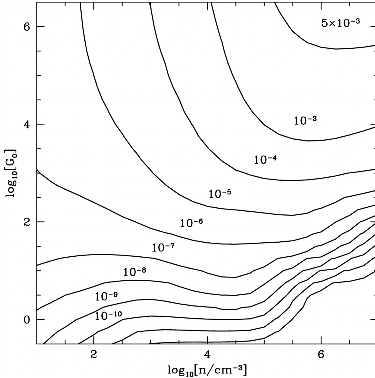
Fig. 1. from [Si II], [Fe II], [C II], and H2 Emission from Massive Starforming Regions Kaufman, Wolfire, & Hollenbach 2006 ApJ 644 283 doi:10.1086/503596 https://dx.doi.org/10.1086/503596
