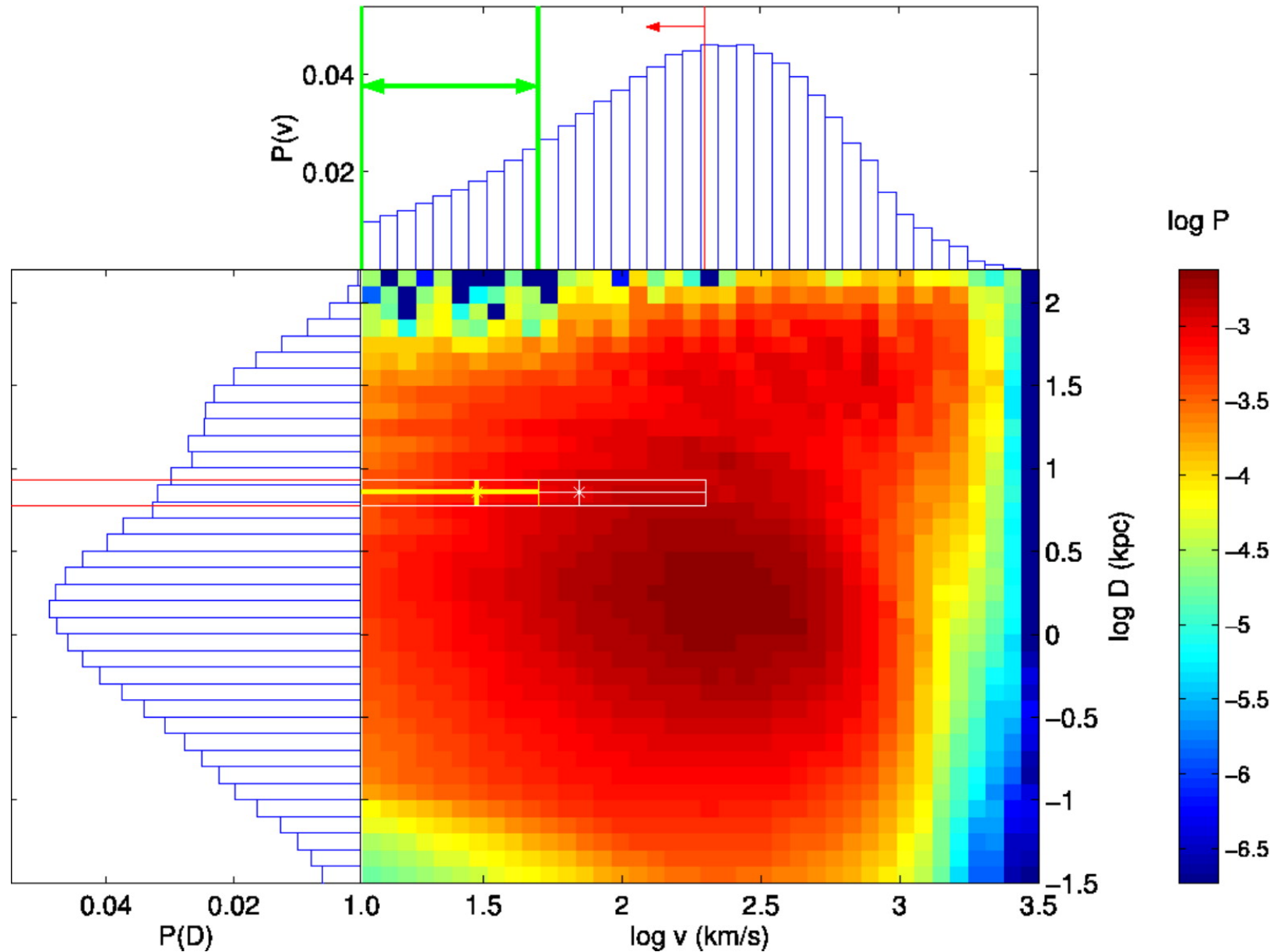
Fig. 2. from ThreeBody Kick to a Bright Quasar Out of Its Galaxy during a Merger Hoffman & Loeb 2006 ApJL 638 L75 doi:10.1086/501230 https://dx.doi.org/10.1086/501230 © 2006. The American Astronomical Society. All rights reserved. Printed in U.S.A.
