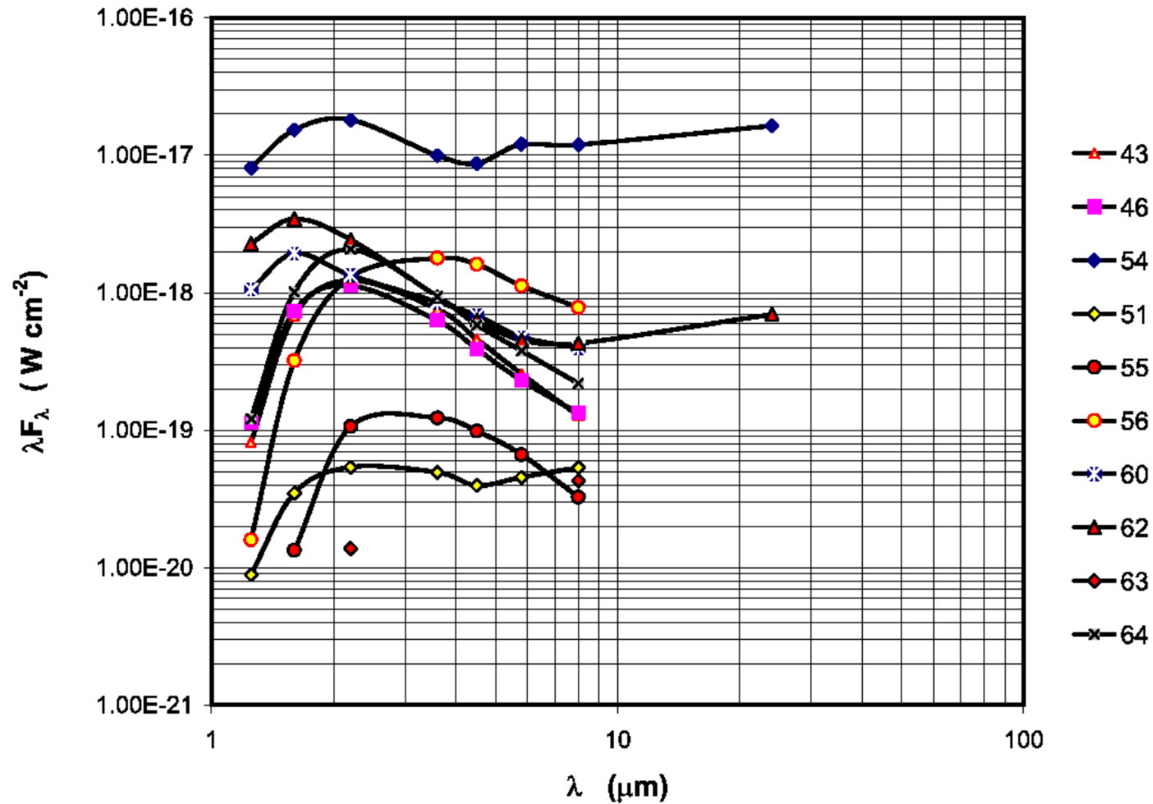
Fig. 7. from Spitzer and Magellan Observations of NGC 2264: A Remarkable Starforming Core near IRS 2 Young et al. 2006 ApJ 642 972 doi:10.1086/501227 https://dx.doi.org/10.1086/501227 © 2006. The American Astronomical Society. All rights reserved. Printed in U.S.A.
